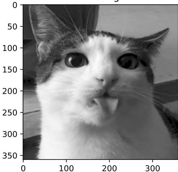
Cat Image
