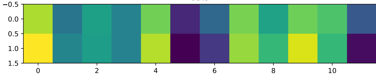
SVD matrices
