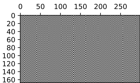
Outer Product
