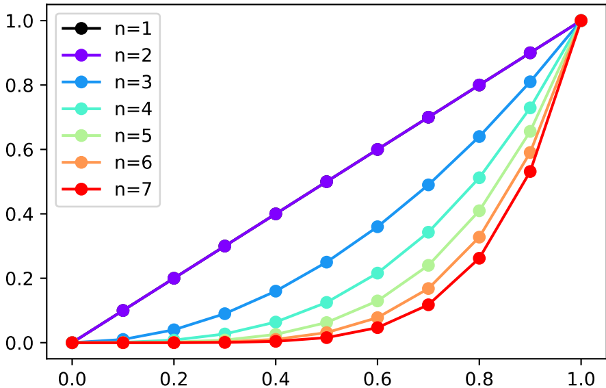
x^n \text{ for } n=1 \text{ to } 7
