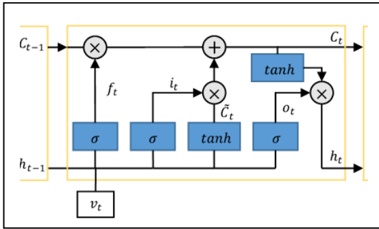
Fig. 3. LSTM architecture
