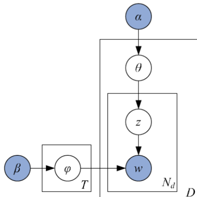
Figure 2: Graphical Model Representation of LDA
