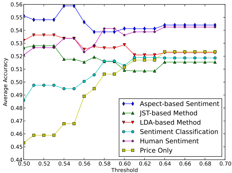
Figure 7: Comparison of the Models for Different Threshold \alpha
