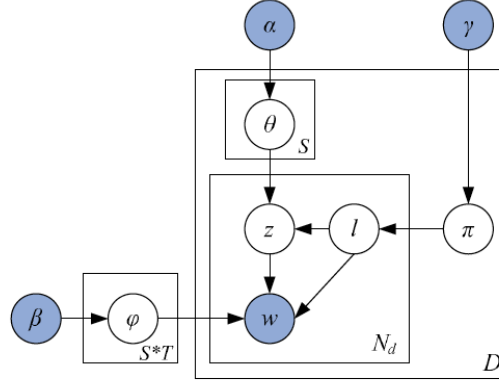
Figure 3: Graphical Model Representation of JST
