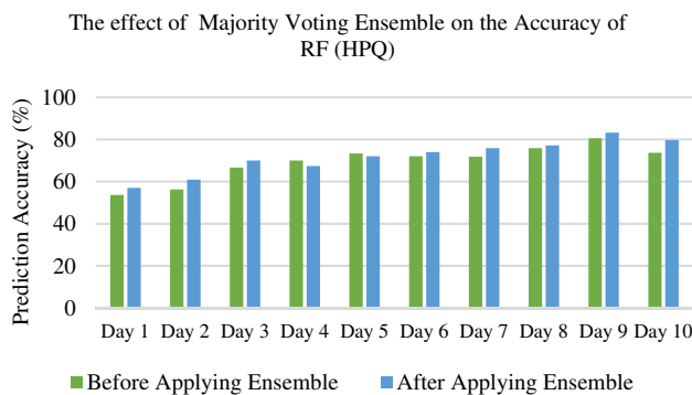
Fig. 18 The effect of VotingClassifier ensemble on the accuracy of RF
