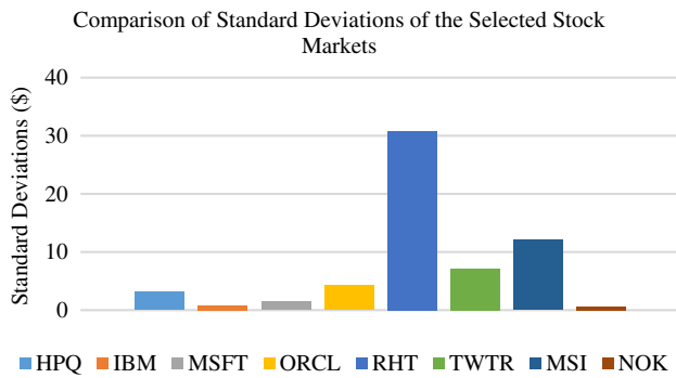
Fig. 13 Comparison of standard deviations for the selected stocks
