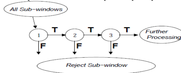
Figure 1: Cascade classifier
