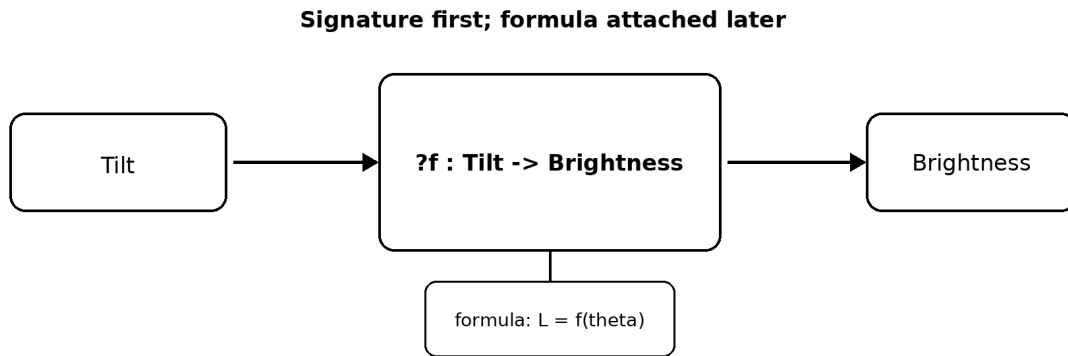
Figure 1: A signature-first relationship. The flow graph contains one semantic relationship, \text{Tilt} \rightarrow \text{Brightness} ; the formula is attached to the block rather than represented as an additional execution step.
