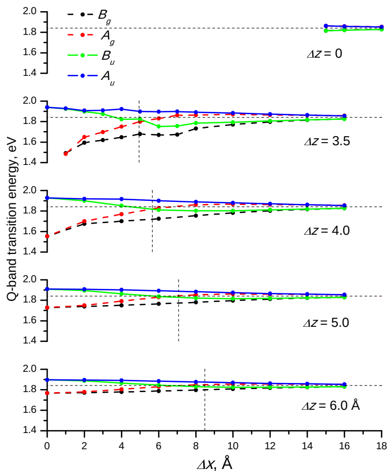
Fig. S1. TD-DFT Q-band transition energies vs. parallel shifts ( \Delta x ) of two Pc molecules (arrangement in Fig. 3B of the main text). Forbidden transitions are shown by dashed lines. Horizontal line represents the Q-band energy of ZnPc, vertical line corresponds to zero-splitting angle of \theta = 54.7^\circ
