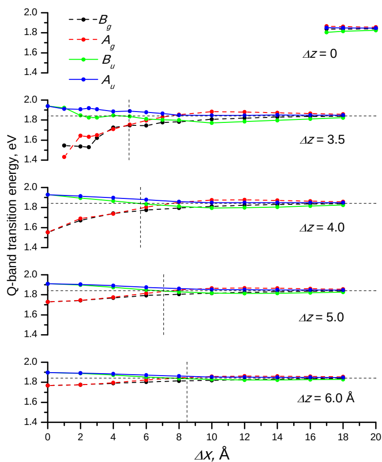
Fig. S2. TD-DFT Q-band transition energies vs. parallel shifts ( \Delta x ) of two Pc molecules (arrangement in Fig. 3A of the main text). Forbidden transitions are shown by dashed lines. Horizontal line represents the Q-band energy of ZnPc, vertical line corresponds to zero-splitting angle of \theta = 54.7^\circ
