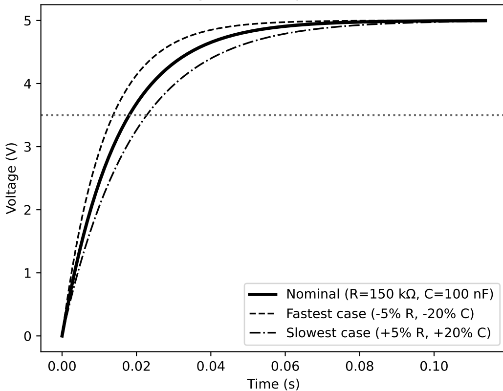
POR timing under component tolerance
