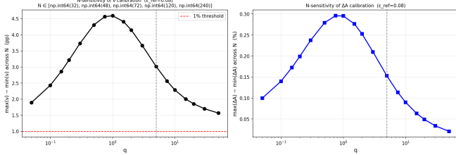
FIG. 6. N -drift \Delta\nu_{\text{meas}} = \max_N \nu_{\text{meas}} - \min_N \nu_{\text{meas}} vs. q at \varepsilon_{\text{ref}} = 0.08 , across N \in \{32, 48, 72, 120, 240\} . The drift peaks near q \approx 1 and exceeds 0.04 across the mid-range squishiness axis, necessitating resolution-matched calibration at the production tier N = 240 .
