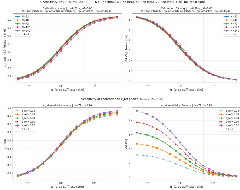
FIG. 5. Top ( N -sensitivity): \nu_{\text{meas}}(q) at \varepsilon_{\text{ref}} = 0.08 for N \in \{32, 48, 72, 120, 240\} . The calibration curve shifts systematically toward lower \nu_{\text{meas}} at fixed q as N increases; the total drift at q = 1 is \Delta\nu_{\text{meas}} = 0.046 from N = 32 to N = 240 . Bottom ( \varepsilon_{\text{ref}} -sensitivity): \nu_{\text{meas}}(q) at N = 72 for \varepsilon_{\text{ref}} \in \{0.04, 0.06, 0.08, 0.10, 0.12\} (bottom to top). Max drift = 0.045 (large q ); the highlighted curve \varepsilon_{\text{ref}} = 0.08 is the working reference.
