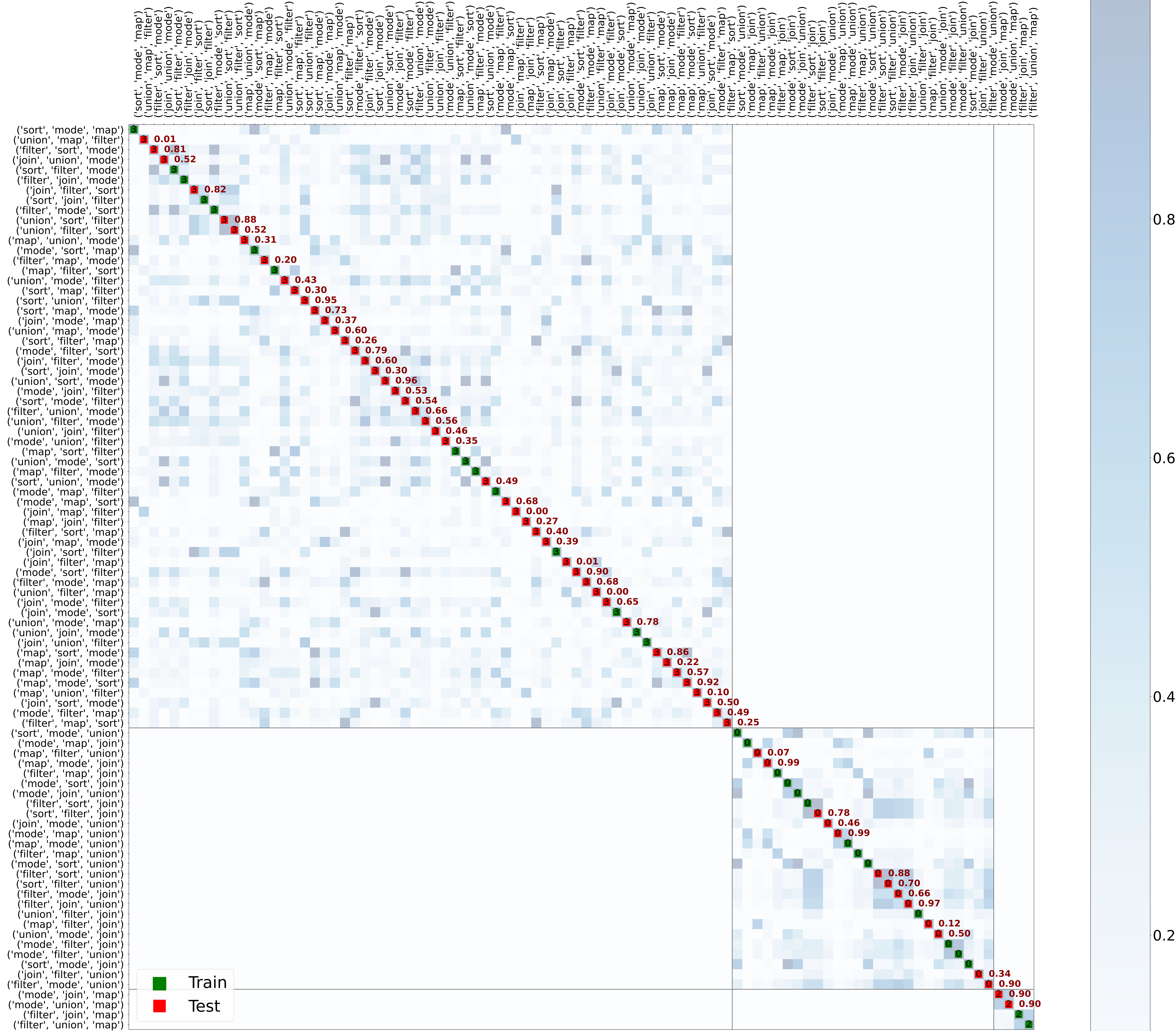
Composition Equivalence Score Matrix, K = 3, Shared Equivalence Classes = 25%
