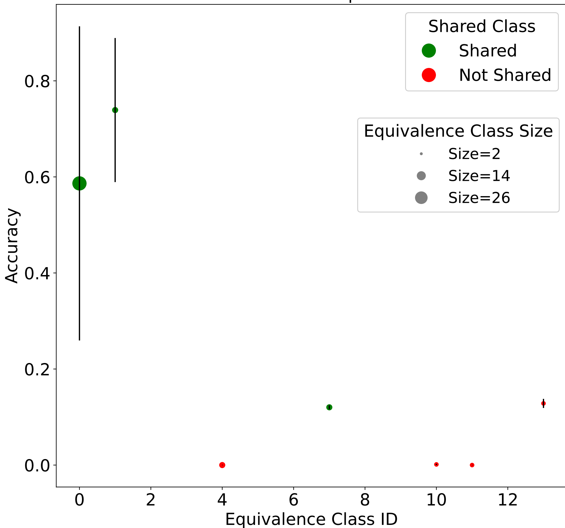
Accuracy distribution for test sequences with and without shared equivalence classes
