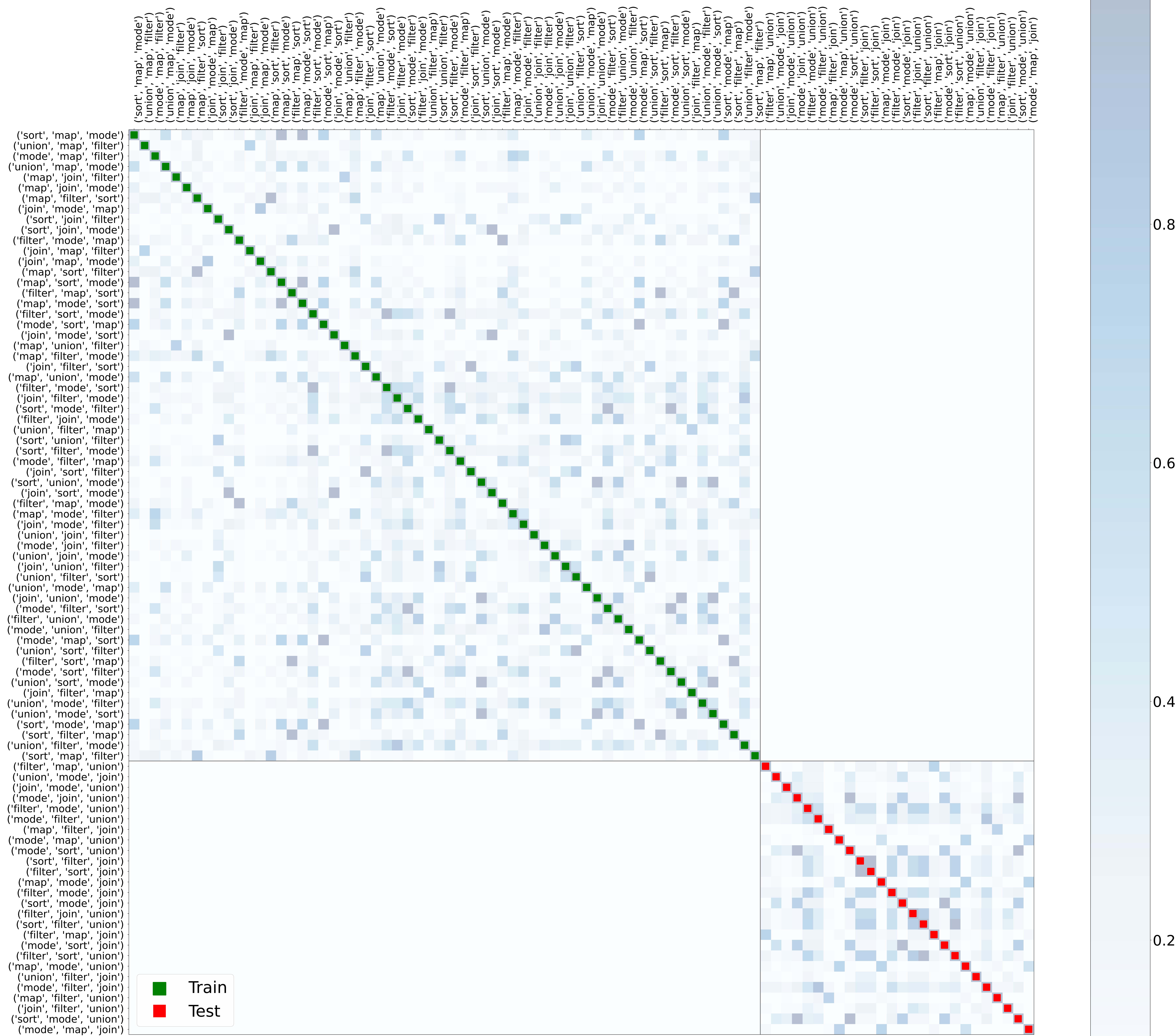
Composition Equivalence Score Matrix, K = 3, Shared Equivalence Classes = 50%
