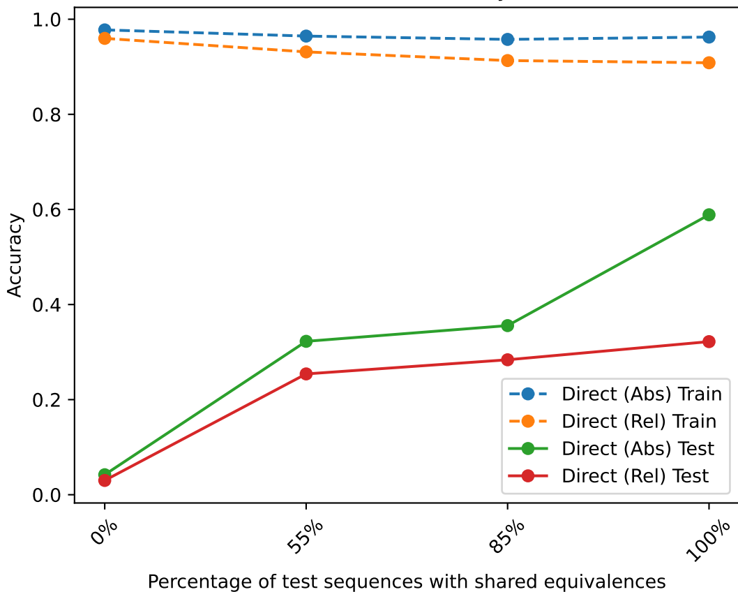
Diverse (without identity), K=3
