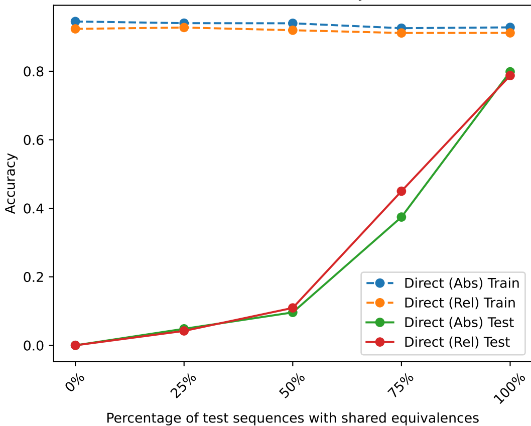
Diverse (without identity), K=6
