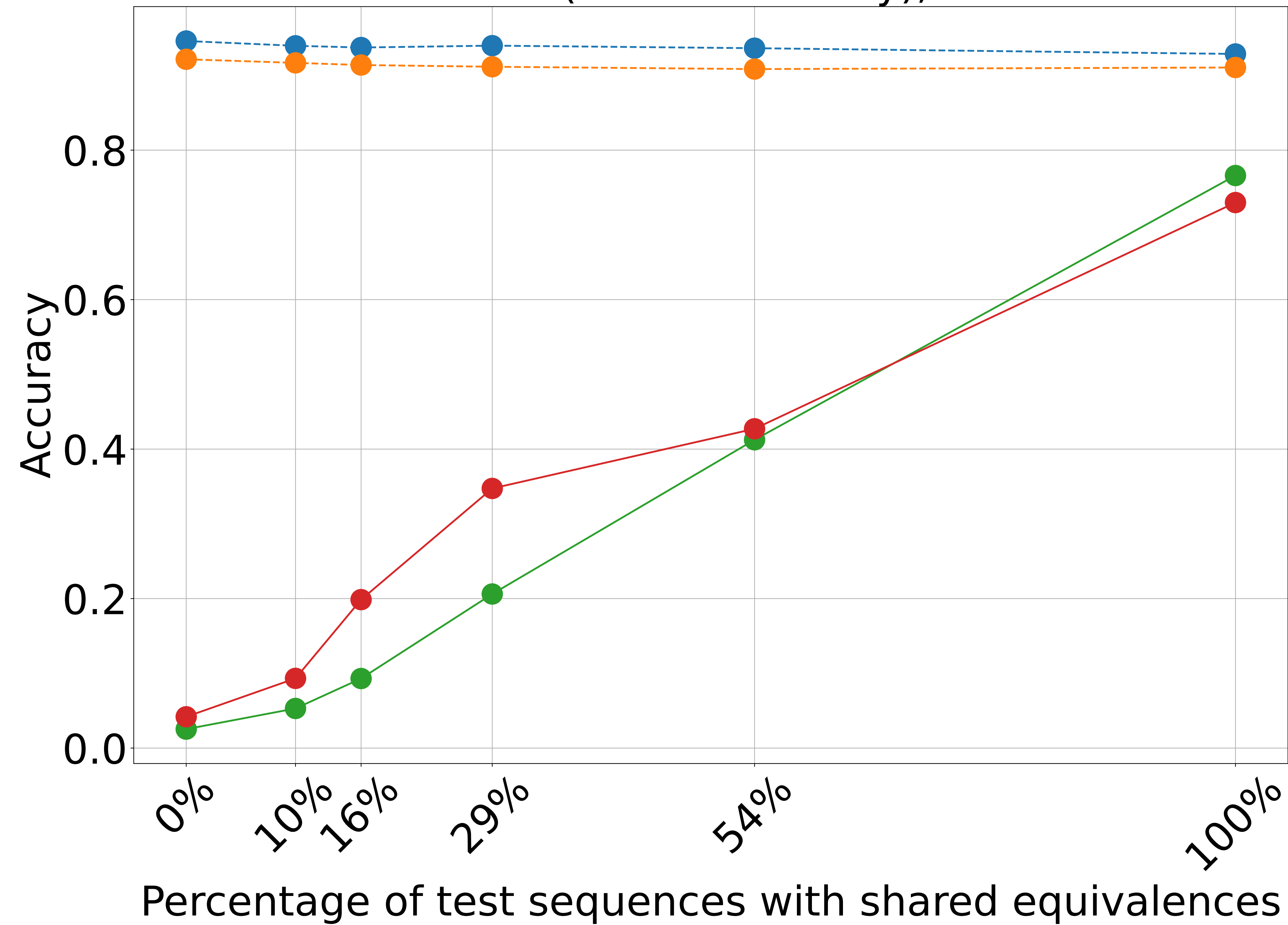
Diverse (without identity), K=6
