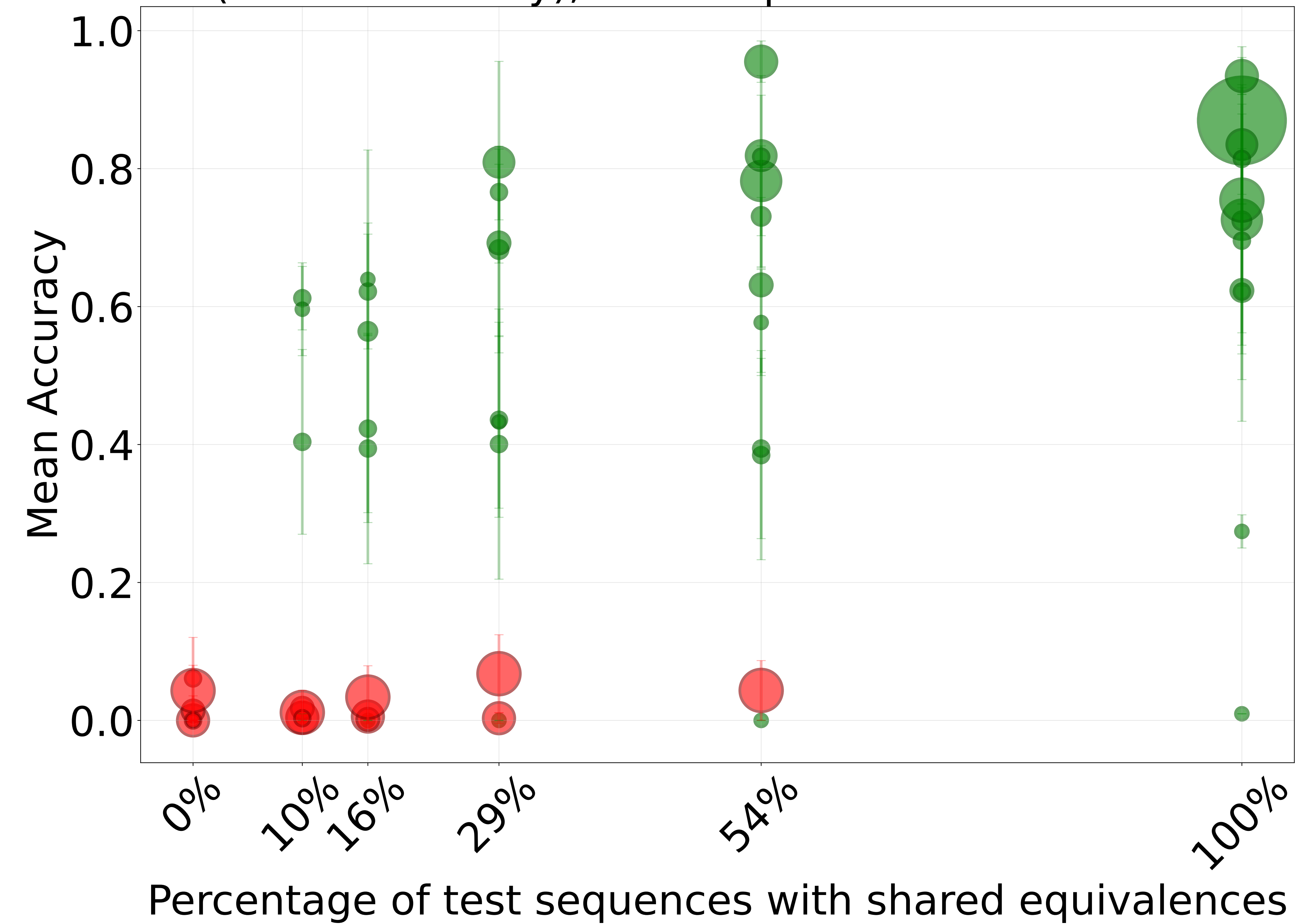
Diverse (without identity), K=6 - Equivalence Classes Distribution
