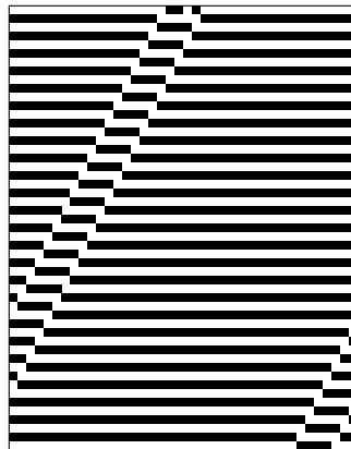
Rule 17
