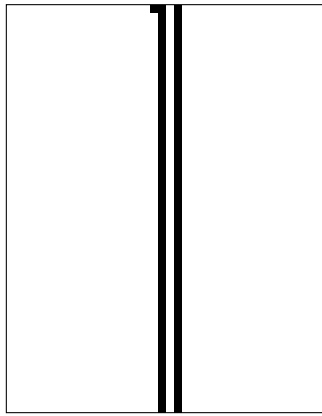
Rule 68
