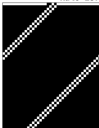
Rule 187
