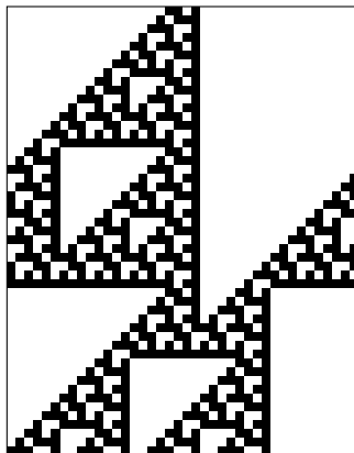
Rule 102
