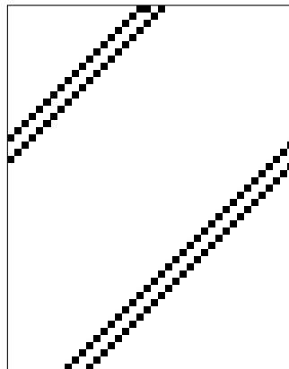
Rule 34
