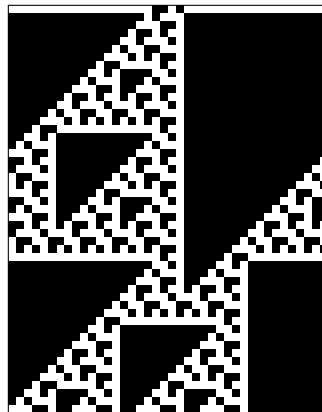
Rule 153
