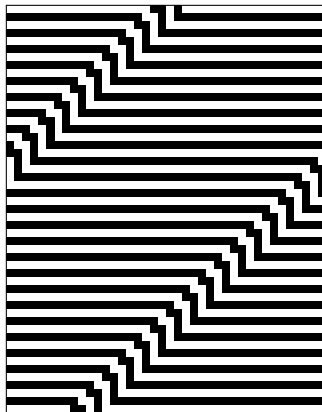
Rule 85
