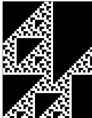
10011001
