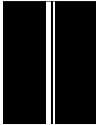
11001100
