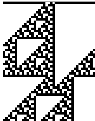
01100110
