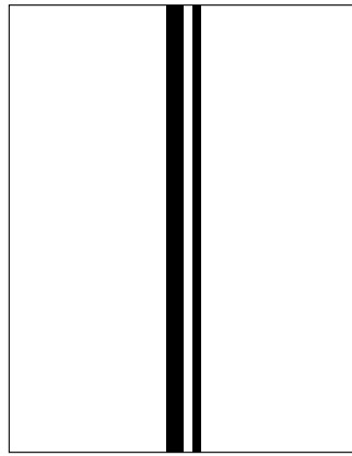
Rule 204
