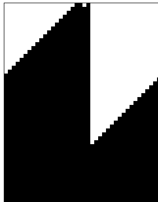
Rule 238
