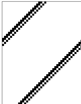
Rule 170
