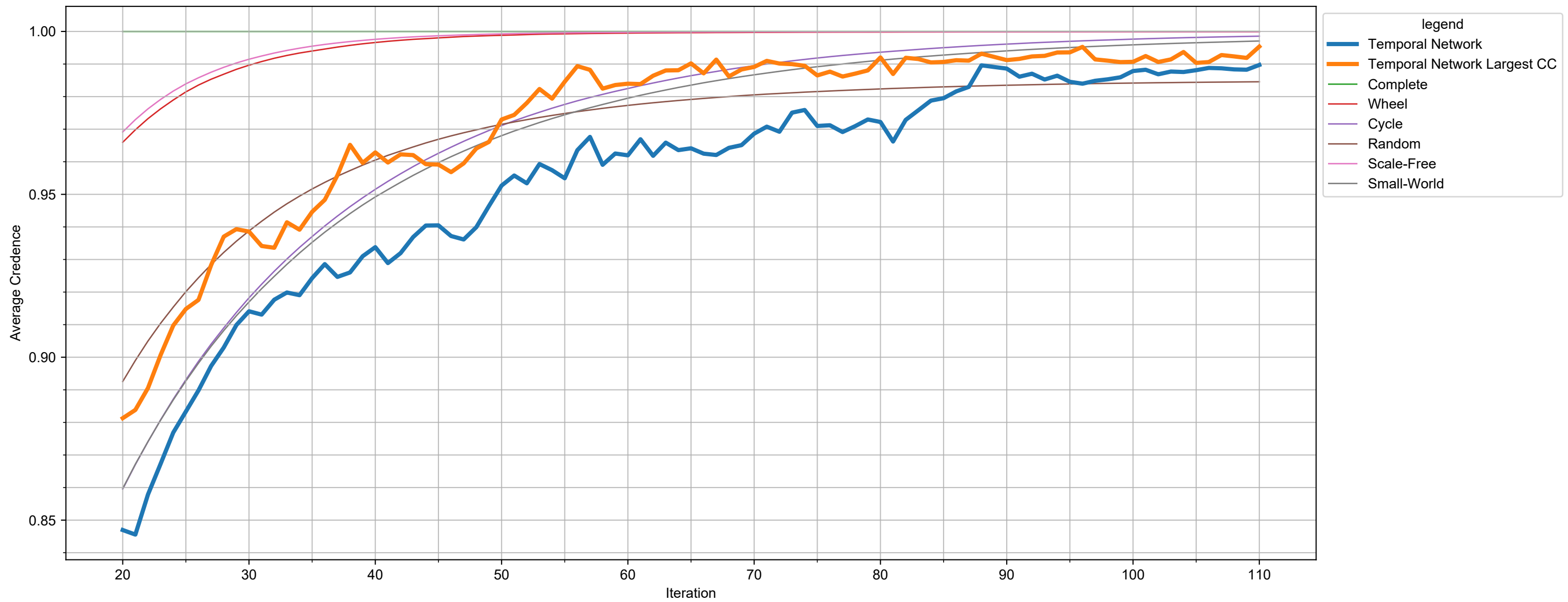
Credence over time
