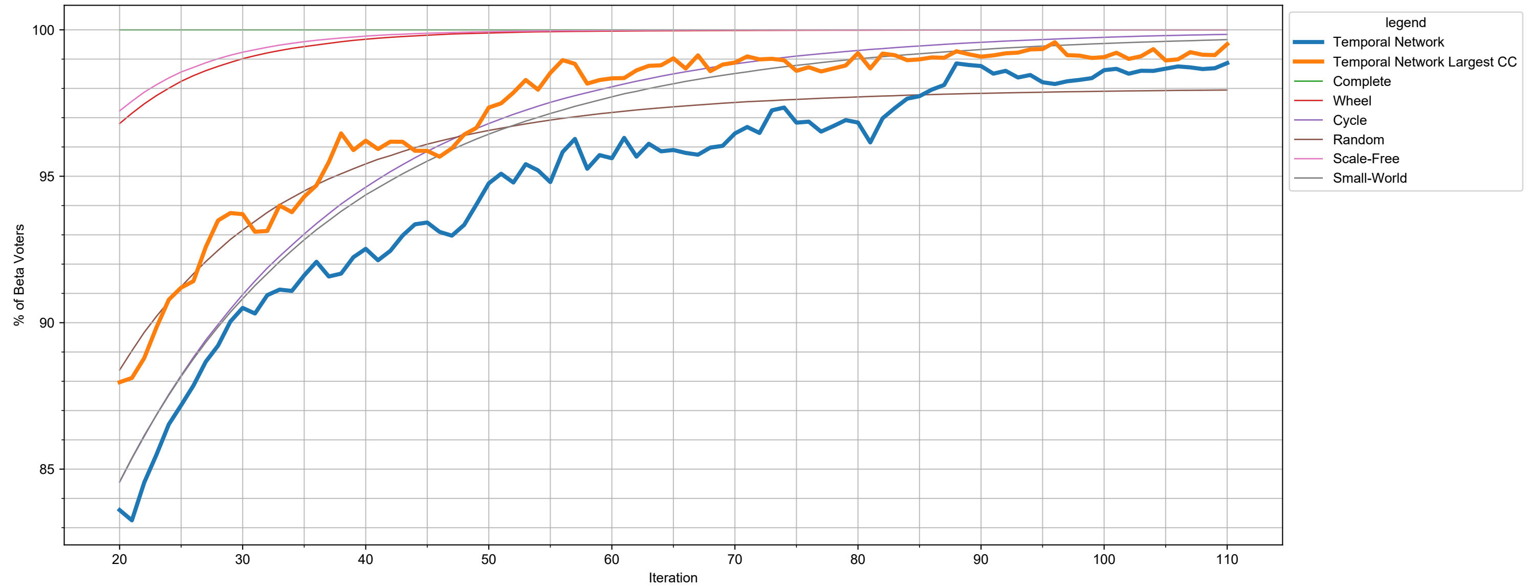
Beta Voters over time
