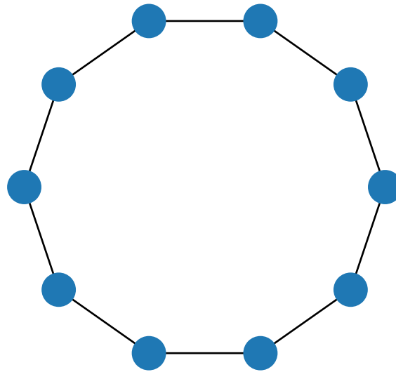
Cycle
