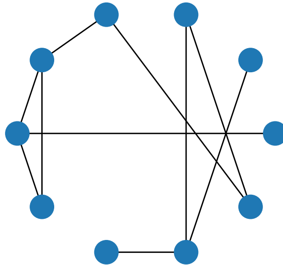
Watts-Strogatz
