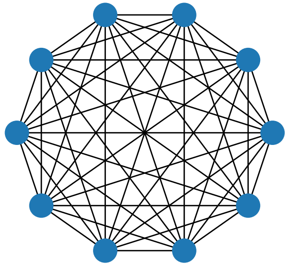
Complete
