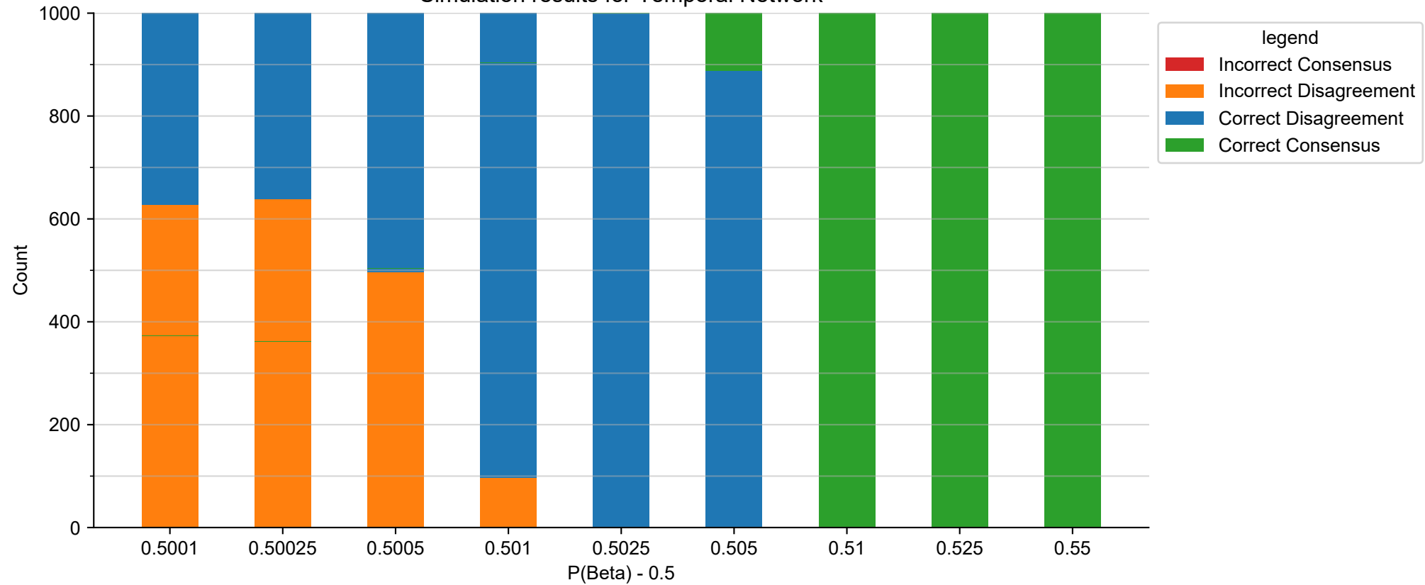
Simulation results for Temporal Network
