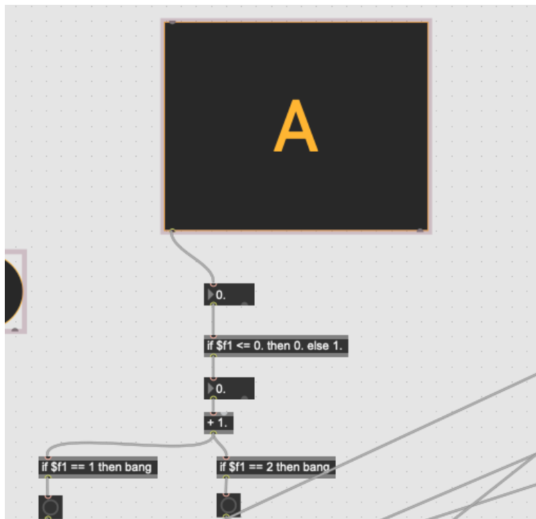
Figure 2.3 – if Statements
