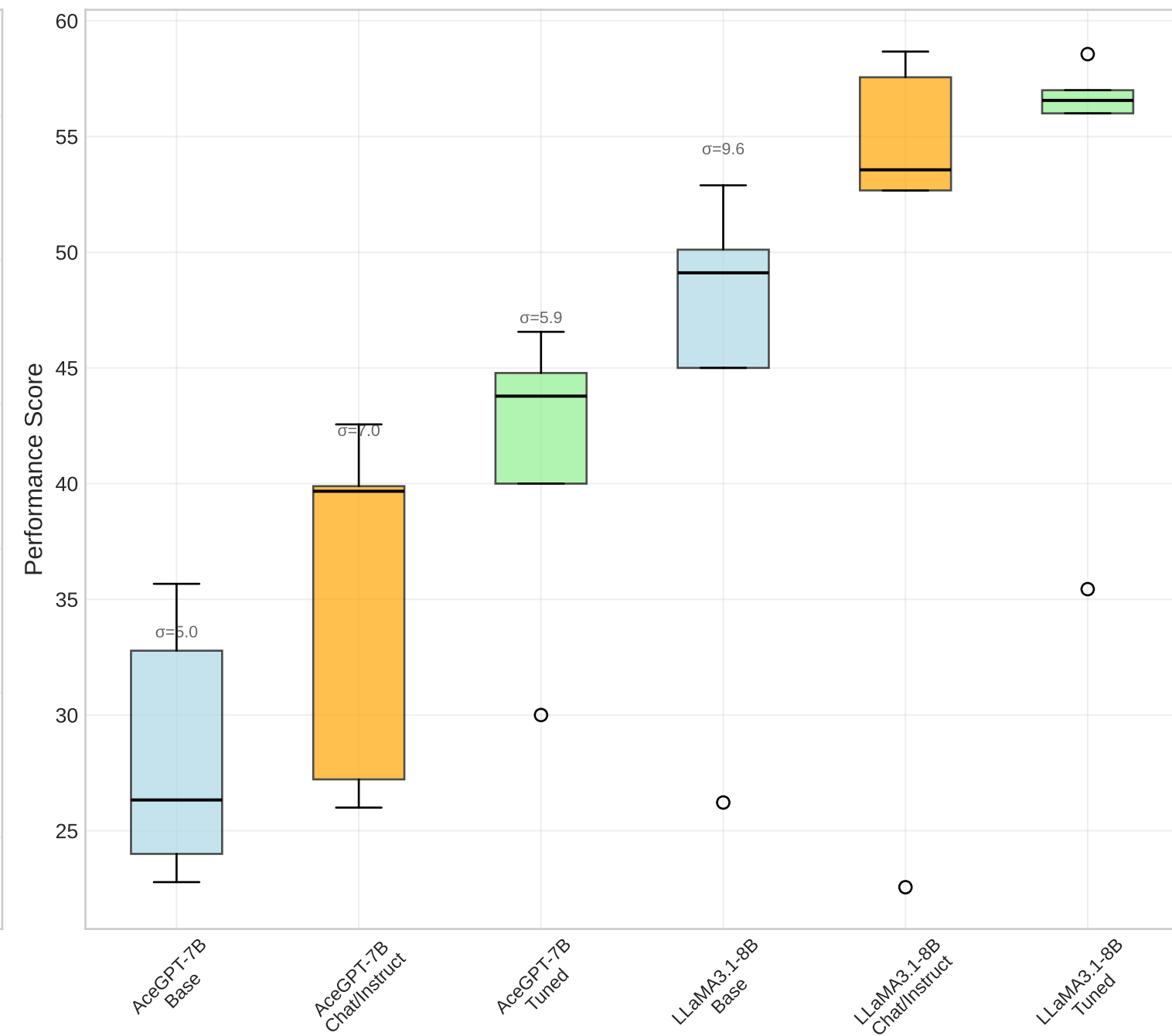
Intra-Task
