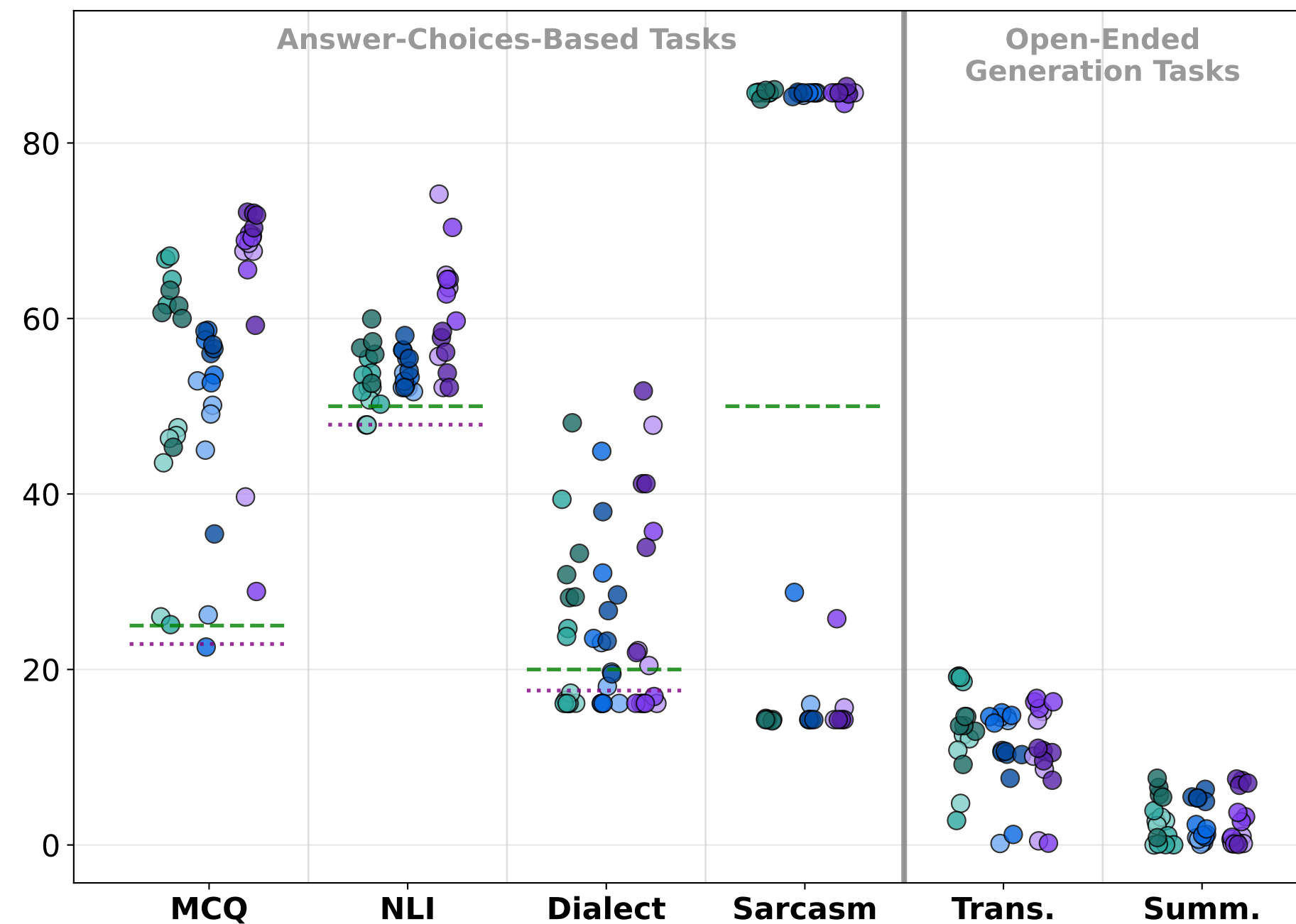
Intra-Task
