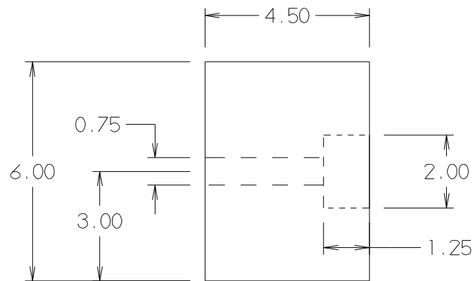
END VIEW 5:1
