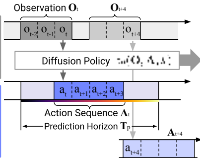
a) Diffusion Policy General Formulation
