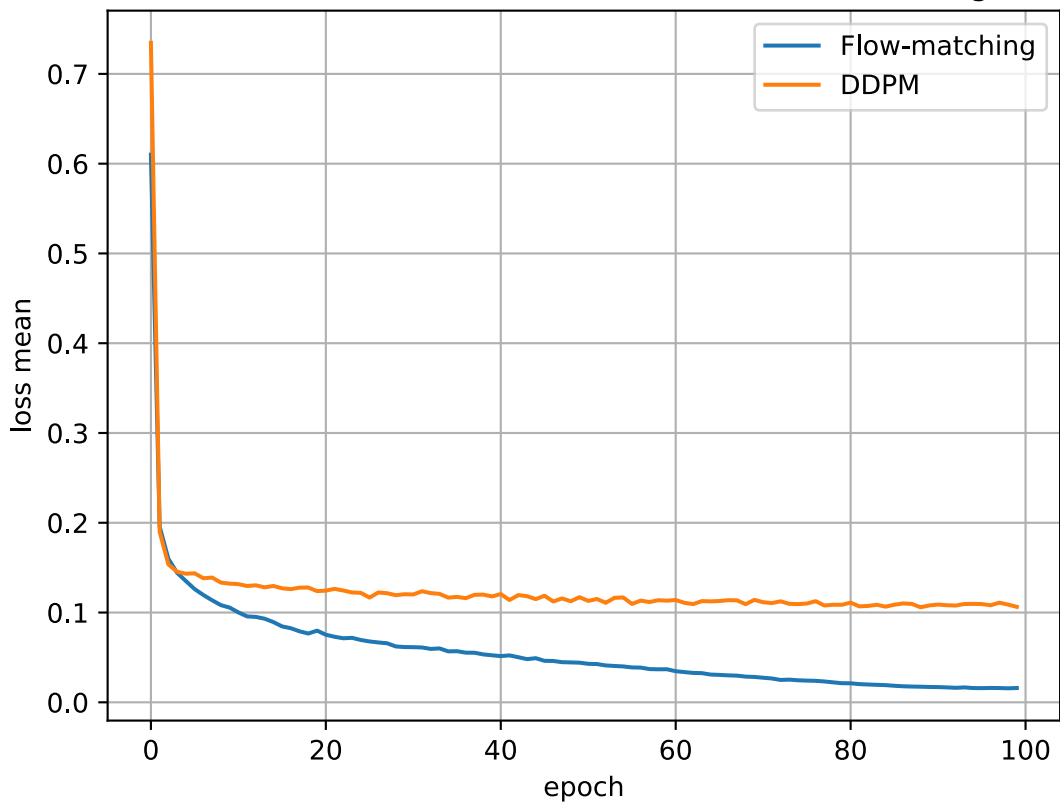
Mean loss for PushT task trained on Flow Matching
