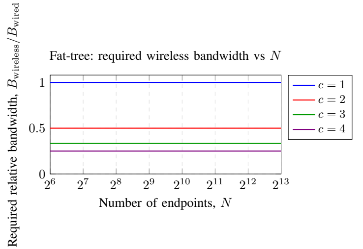
Fig. 2: Fat-tree connection-limited required minimum relative bandwidth. The required bandwidth is 1/c , independent of N , so it appears as a flat horizontal line for each value of c .
