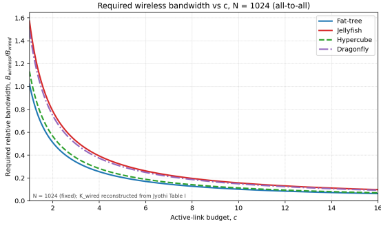
Fig. 6: Mode 1 (all-to-all): required minimum B_{\text{wireless}}/B_{\text{wired}} vs c at N = 1024 . The required bandwidth is K_{\text{wired}}(N-1)/c . At N = 1024 , the absolute values are comparable to mode 0, but the all-to-all required bandwidth grows with N , so all-to-all becomes increasingly demanding at large scale.
