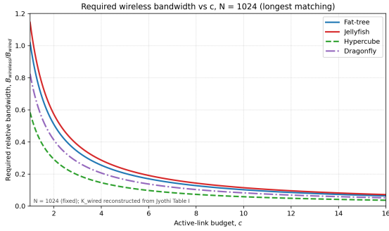
Fig. 7: Mode 4 (longest matching): required minimum B_{\text{wireless}}/B_{\text{wired}} vs c at N = 1024 . The required bandwidth is K_{\text{wired}}/c . Hypercube has a notably lower required bandwidth than the other topologies because its longest-matching K_{\text{wired}} is low.
