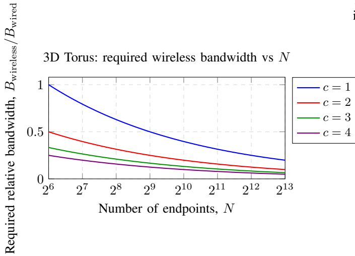
Fig. 4: 3D Torus connection-limited required minimum relative bandwidth. The required bandwidth 4/(cN^{1/3}) decreases with N , unlike Fat-tree and Hypercube, because the Torus bisection width grows faster than linearly in N .
