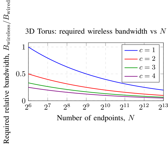
Fig. 4: 3D Torus connection-limited required minimum relative bandwidth. The required bandwidth 4/(cN^{1/3}) decreases with N , unlike Fat-tree and Hypercube, because the Torus bisection width grows faster than linearly in N .
