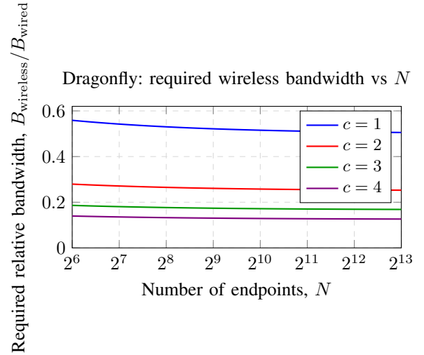
Fig. 3: Dragonfly connection-limited required minimum relative bandwidth. The required bandwidth converges to 1/(2c) for large N due to the group-level cut structure.
