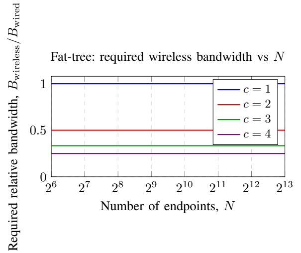
Fig. 2: Fat-tree connection-limited required minimum relative bandwidth. The required bandwidth is 1/c , independent of N , so it appears as a flat horizontal line for each value of c .
