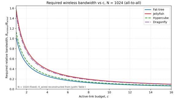
Fig. 6: Mode 1 (all-to-all): required minimum B_{\text{wireless}}/B_{\text{wired}} vs c at N = 1024 . The required bandwidth is K_{\text{wired}}(N-1)/c . At N = 1024 , the absolute values are comparable to mode 0, but the all-to-all required bandwidth grows with N , so all-to-all becomes increasingly demanding at large scale.
