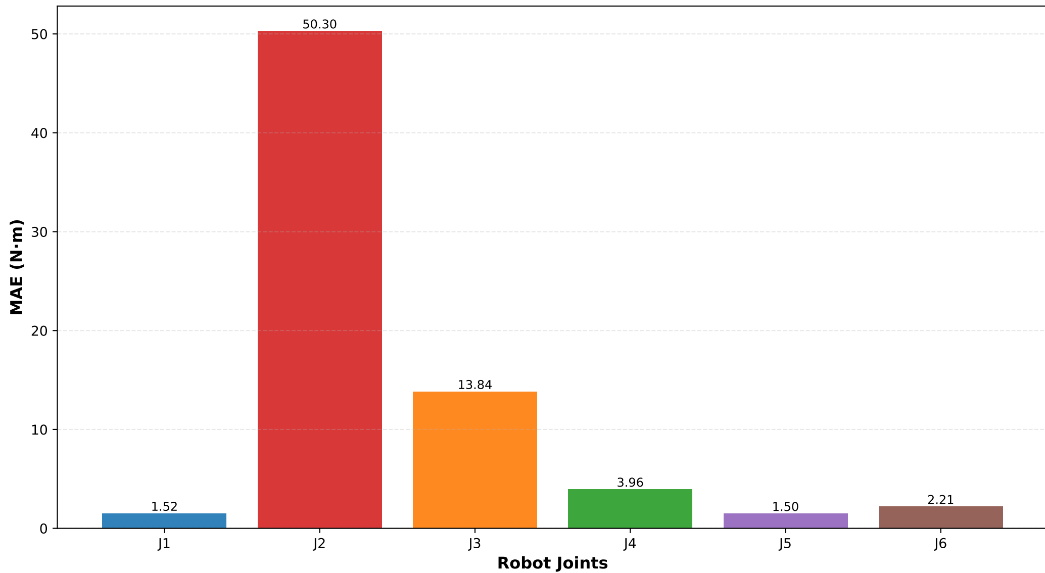
Per-Joint MAE (CNN vs PD Targets)
