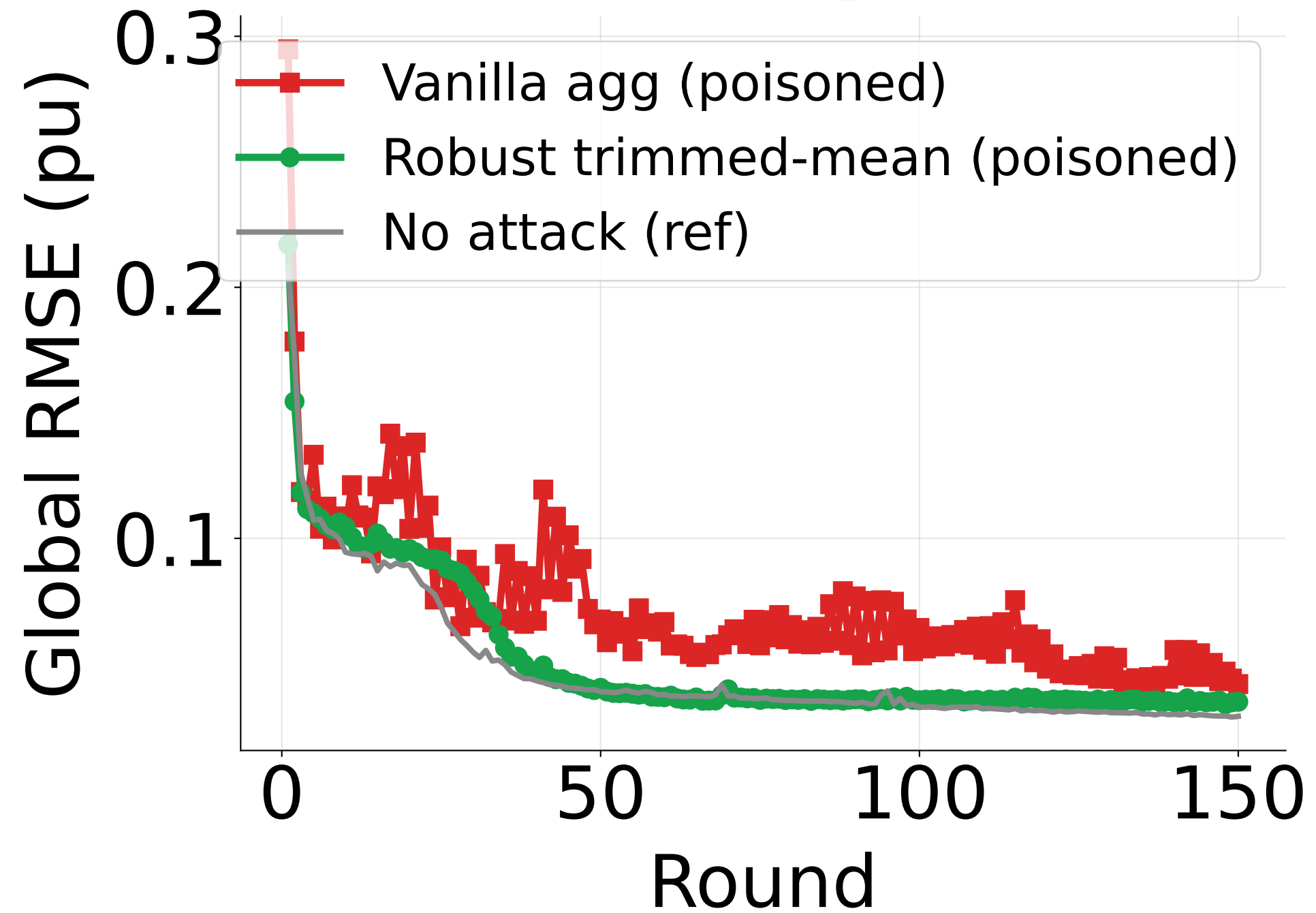
(b) Robustness to a poisoned client
