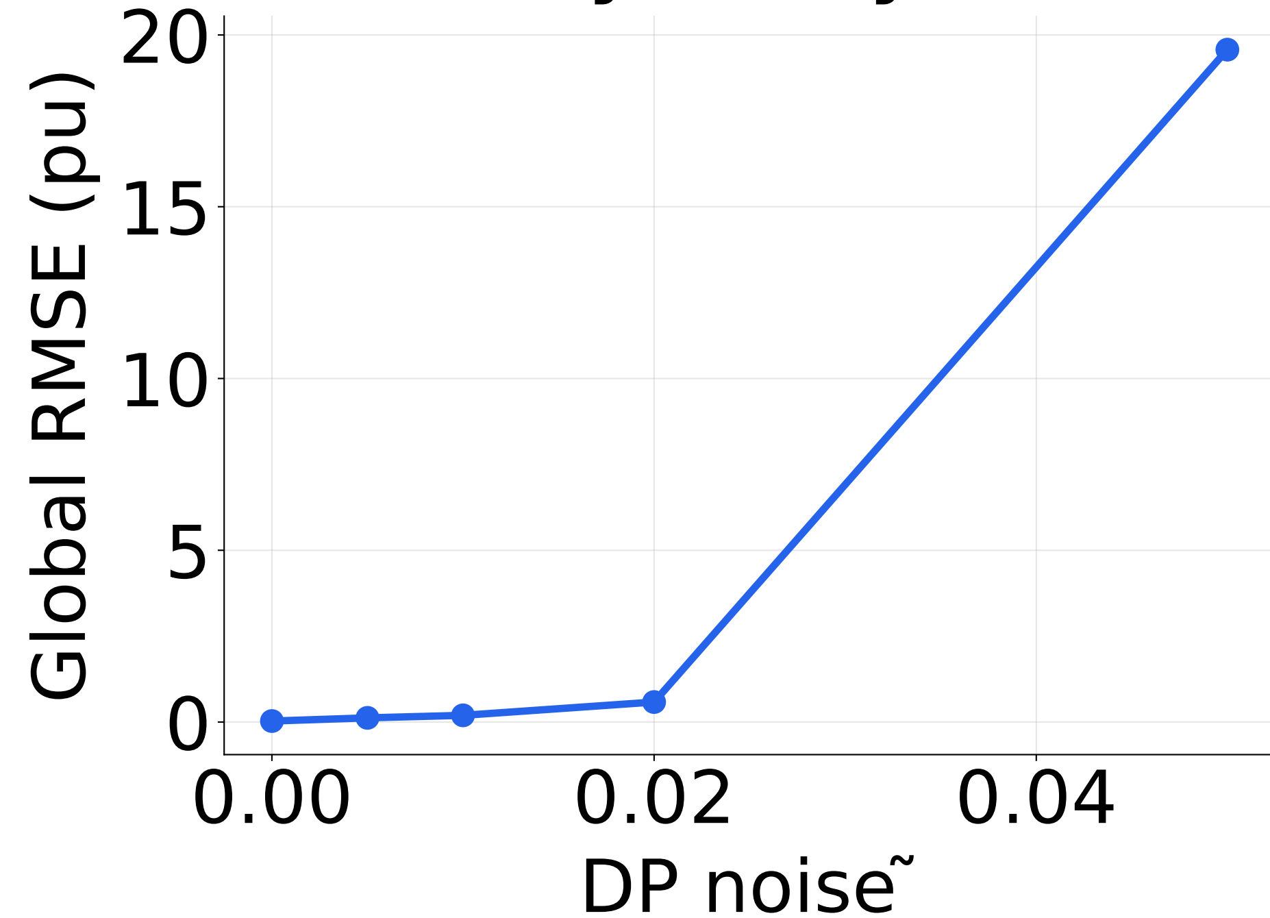
(a) Privacy-utility trade-off
