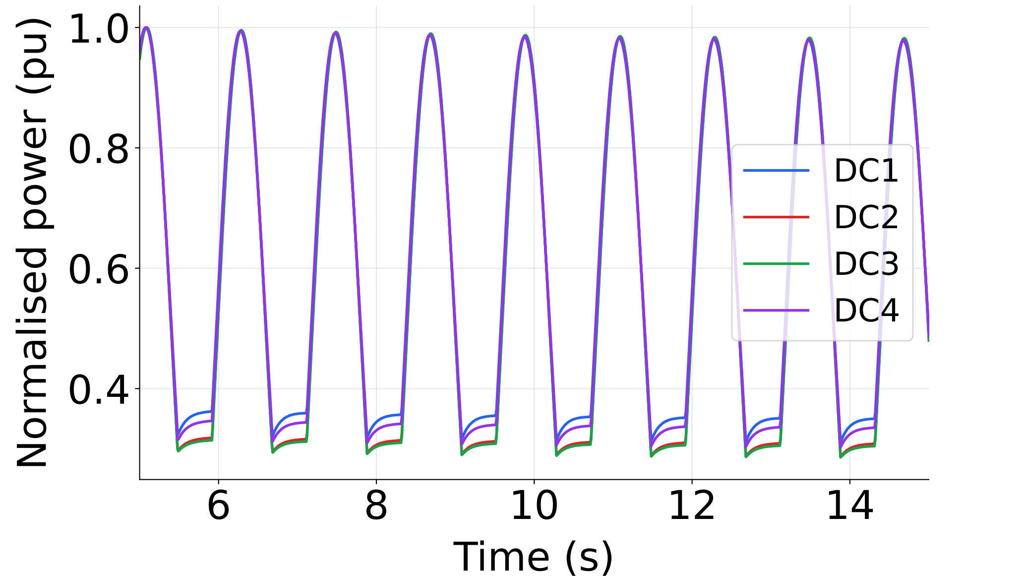
(b) Locally-normalised (privacy-preserving)
