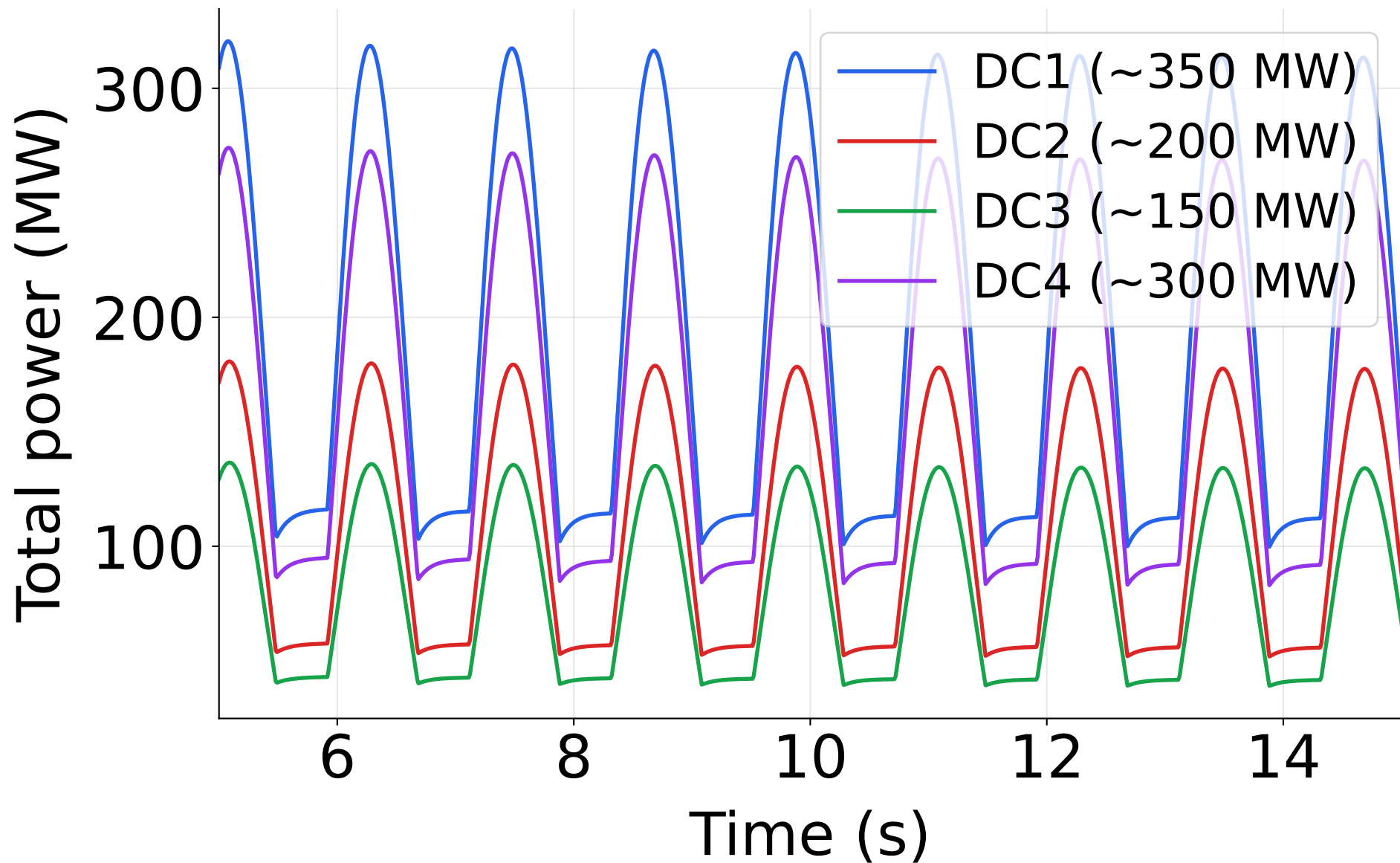
(a) Measured DC load profiles
