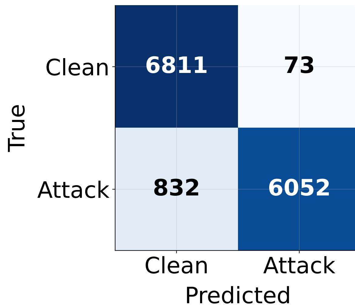
Confusion matrix
