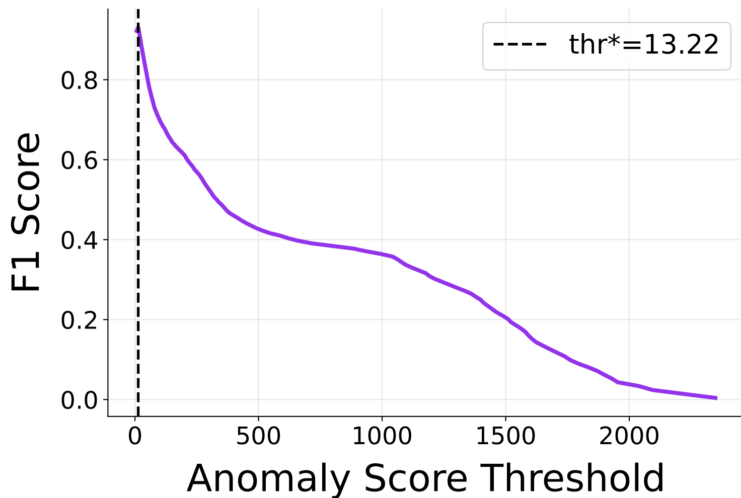
Threshold tuning (max F1=0.930)
