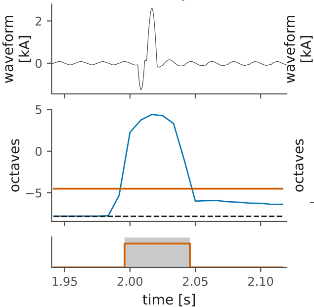
(a) record 907: 1-cycle BC fault
