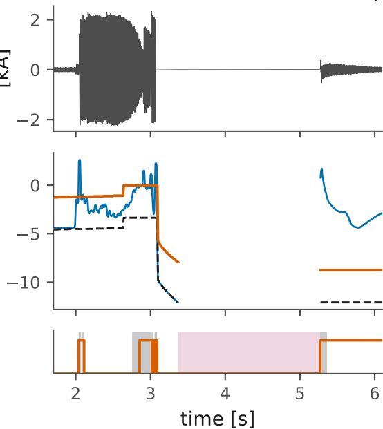
(b) record 677: ABG fault, 2.2 s open, reclose
