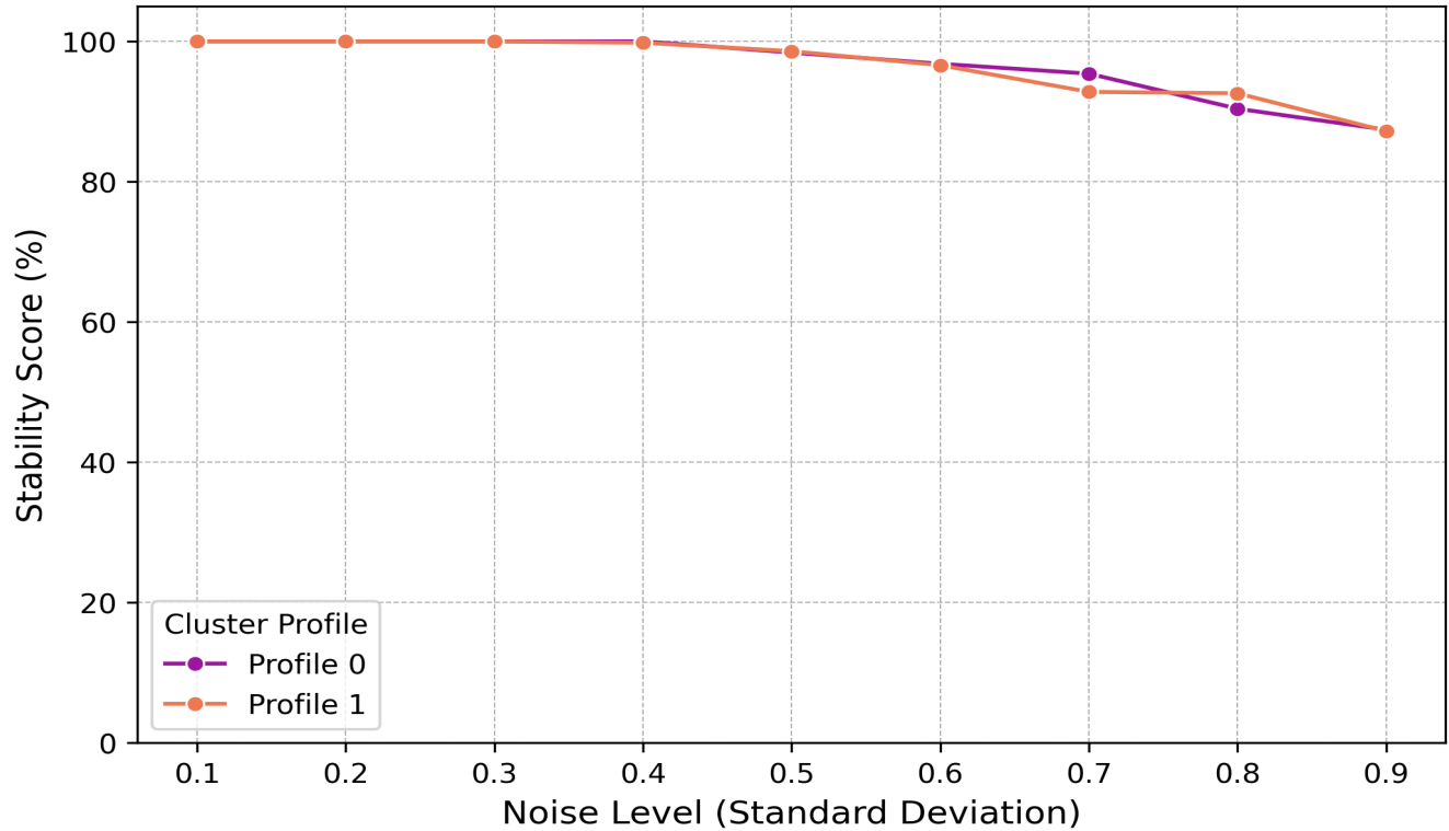
Stability Profile for DDoS-HOIC Clusters
