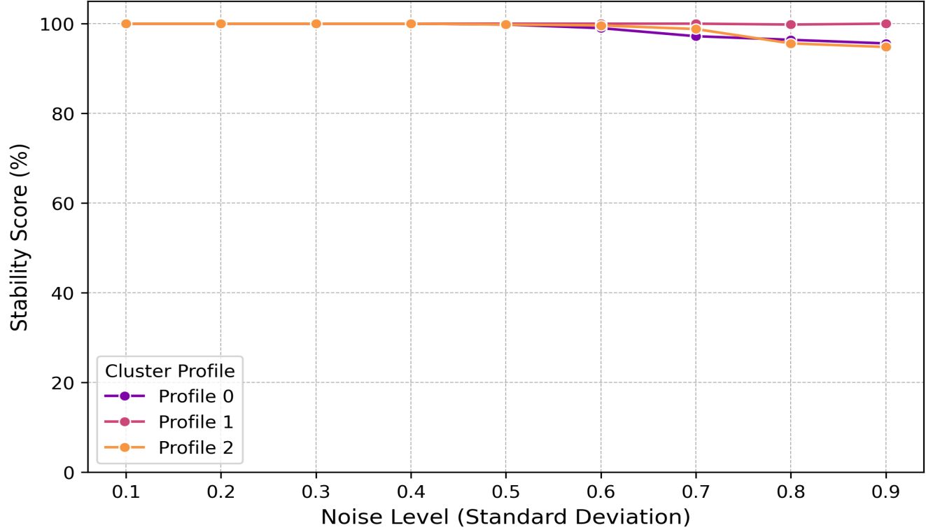
Stability Profile for DoS-Hulk Clusters
