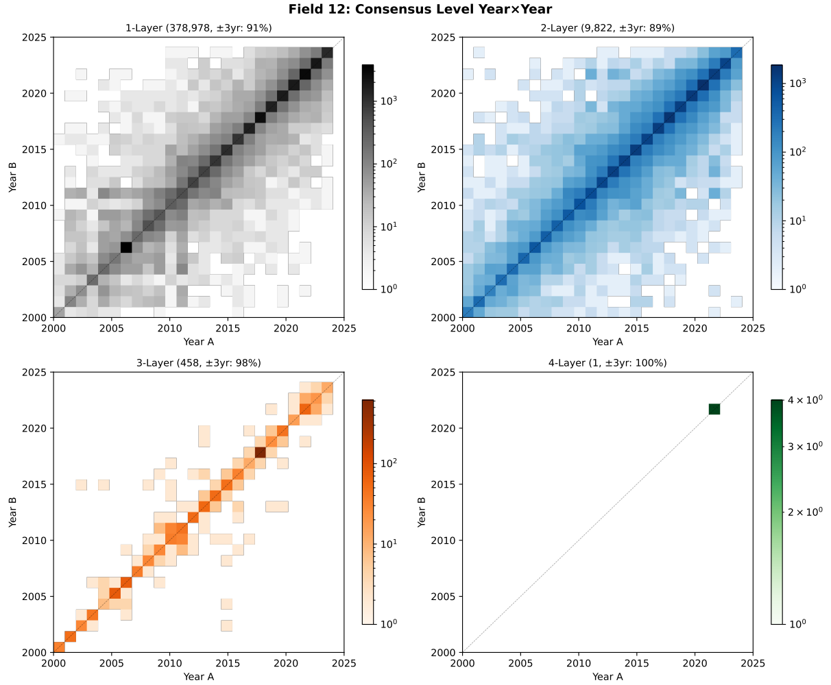
Figure 10: Field 12 consensus levels. Even 1-layer edges are highly diagonal (91%) due to sparse, temporally narrow citation patterns. 3-layer achieves 98% but contains only 458 edges.
