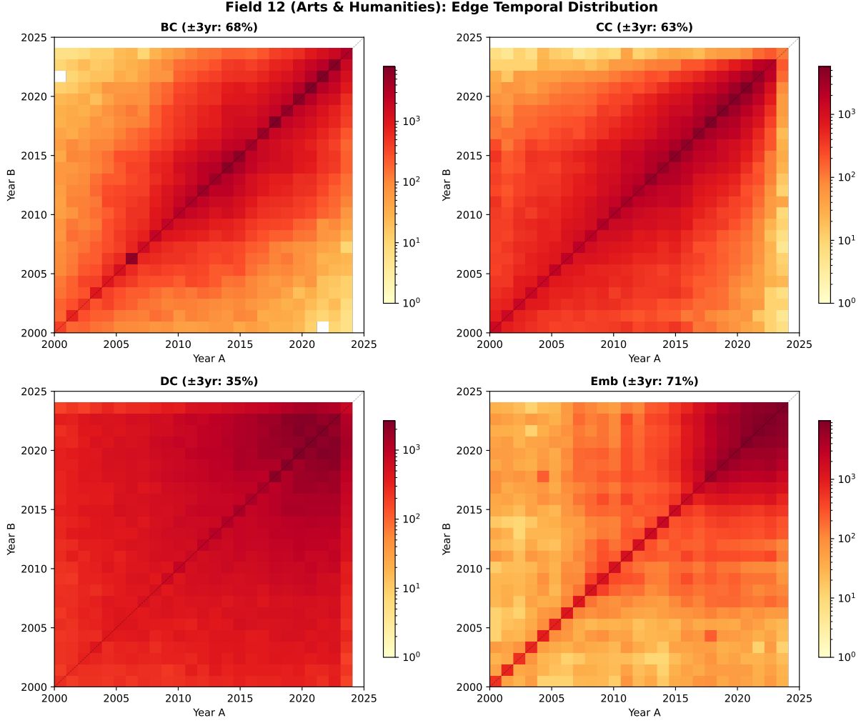
Figure 9: Field 12 edge landscape. DC is extremely broad (35% diagonal); Emb is the most diagonal-concentrated (71%), reversing the Field 15 pattern.
