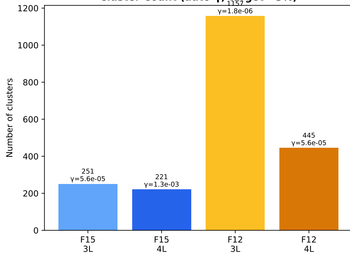
Cluster Count (auto- \gamma , target <3%)
