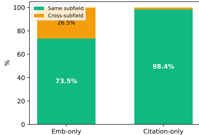
Subfield Match Rate
