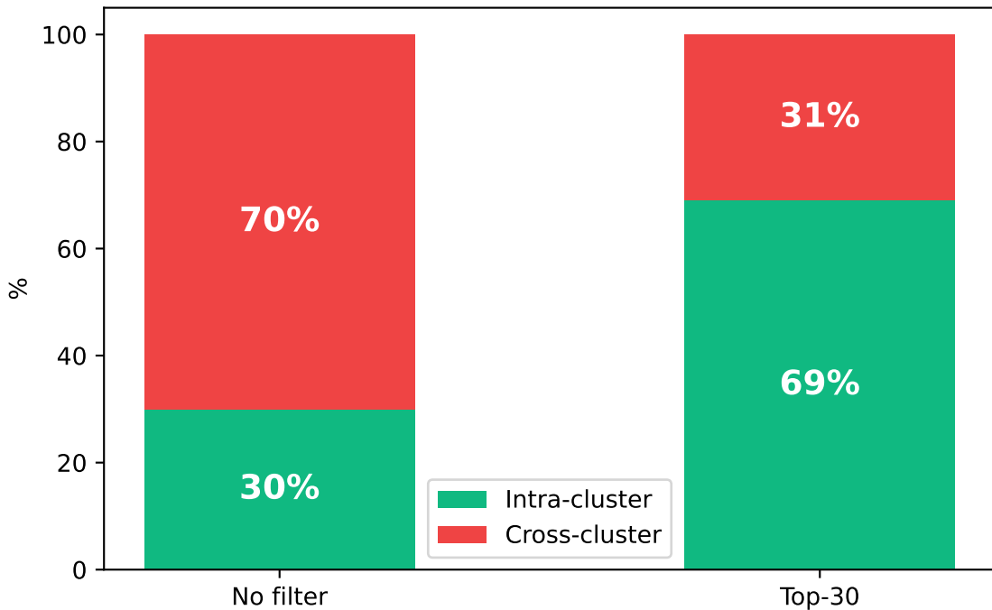
Top-k Filter Effect on Cross-cluster Edges
