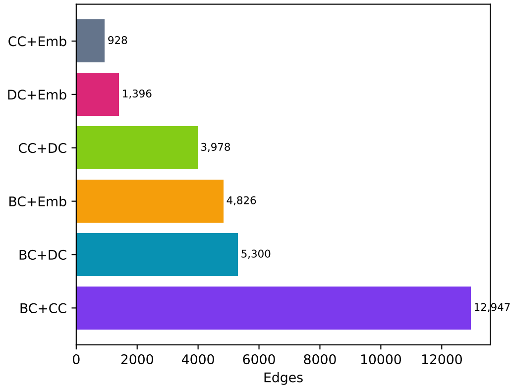
2-Layer consensus
