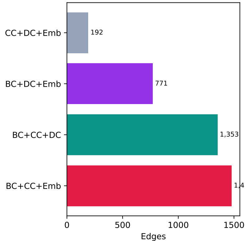
3-Layer consensus
