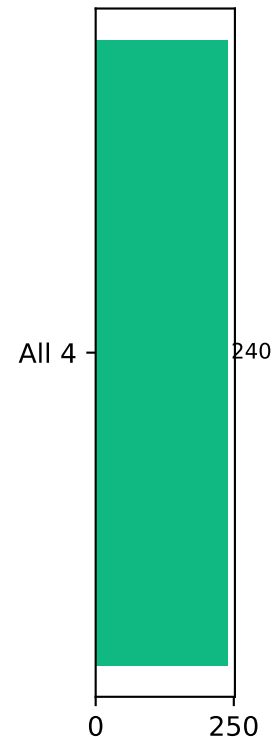
4-Layer full
