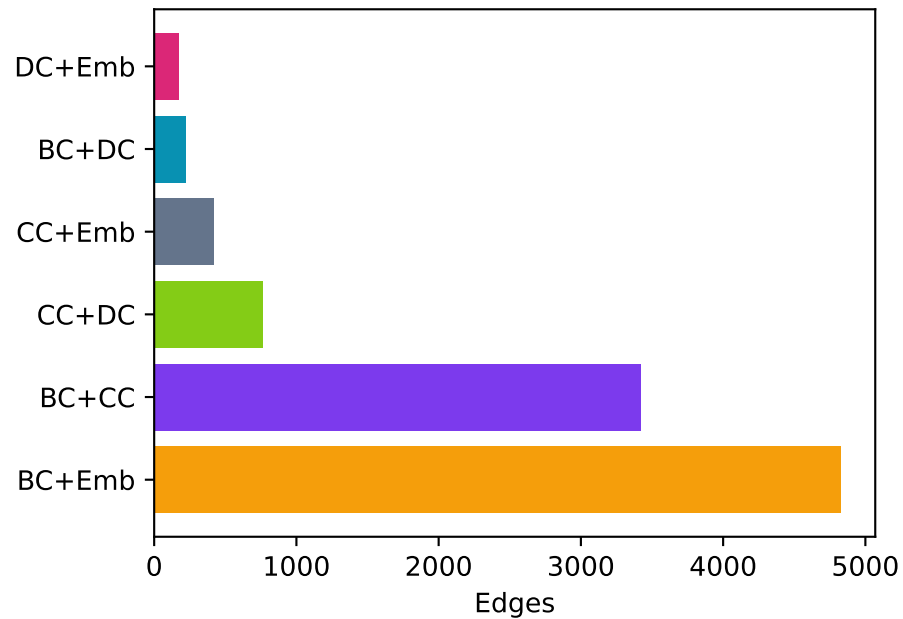
2-Layer (2.5%)
