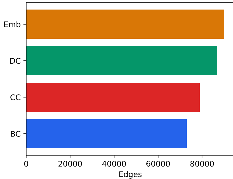
1-Layer (97.4%)
