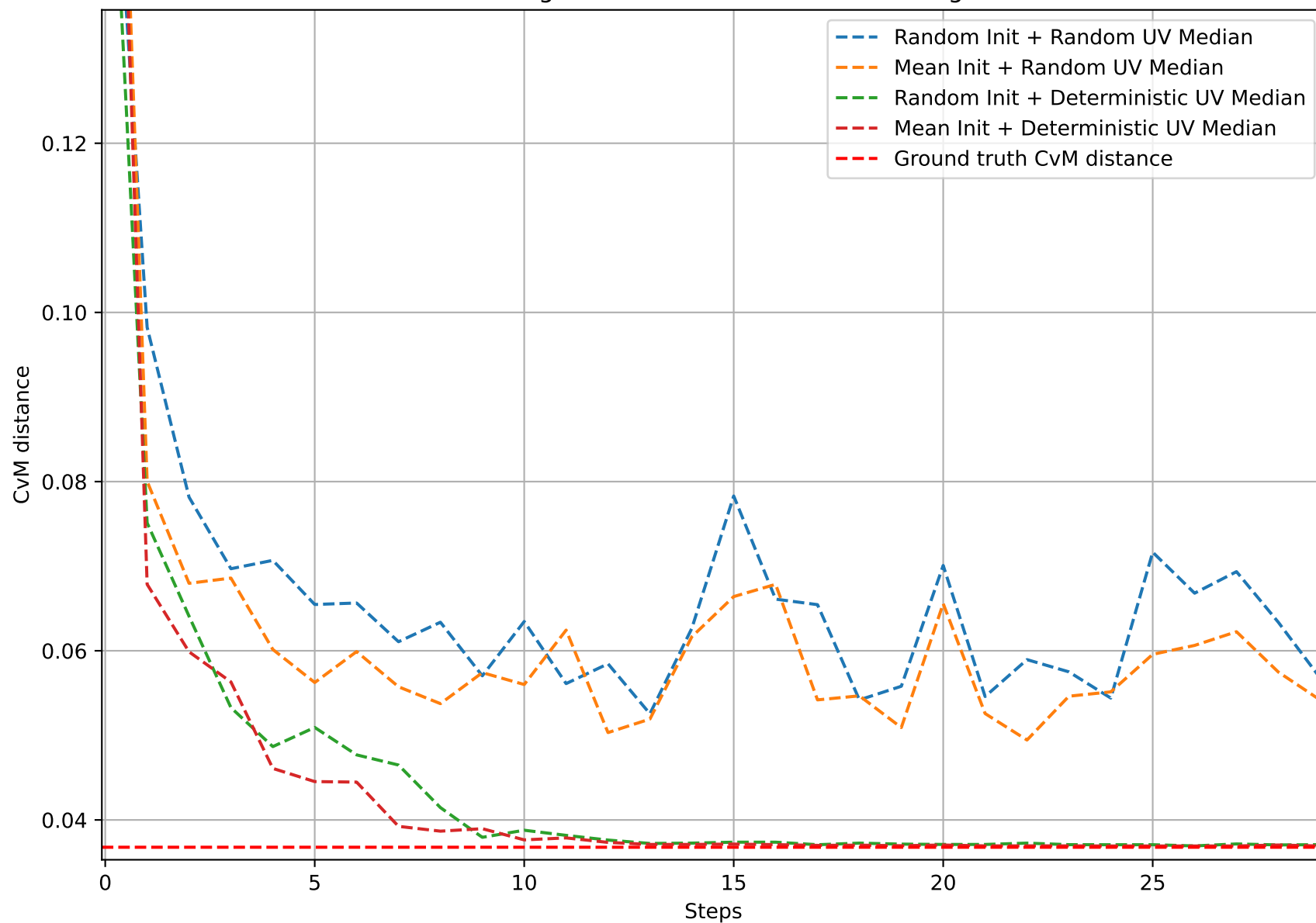
Convergence of PCD with different configs
