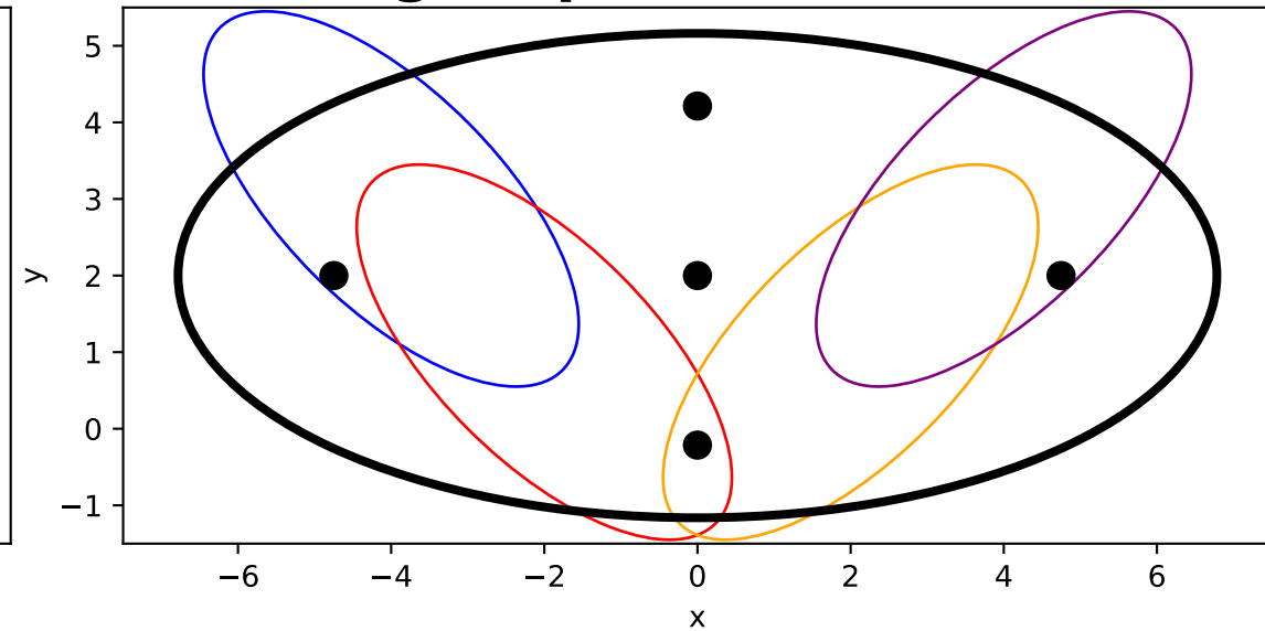
Unscented sigma points (reduced Gaussian)
