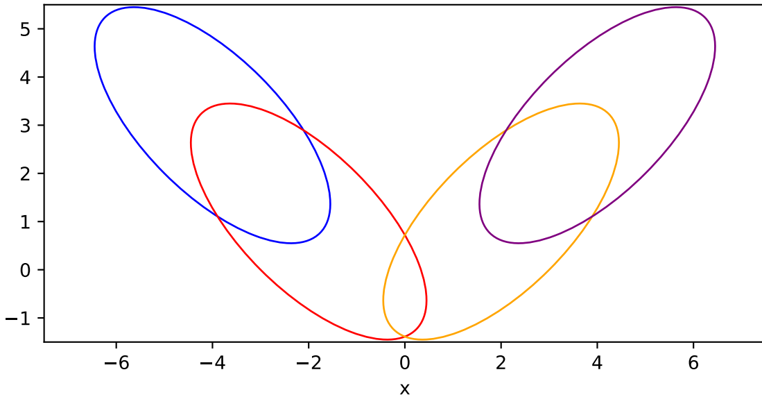
Original 4-component GMM
