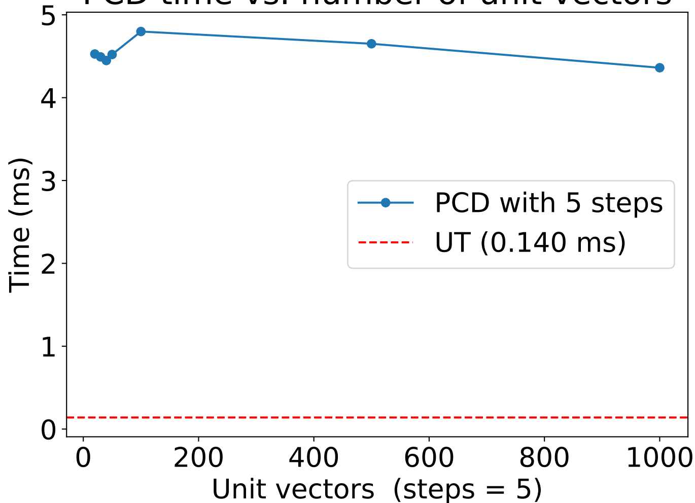
PCD time vs. number of unit vectors
