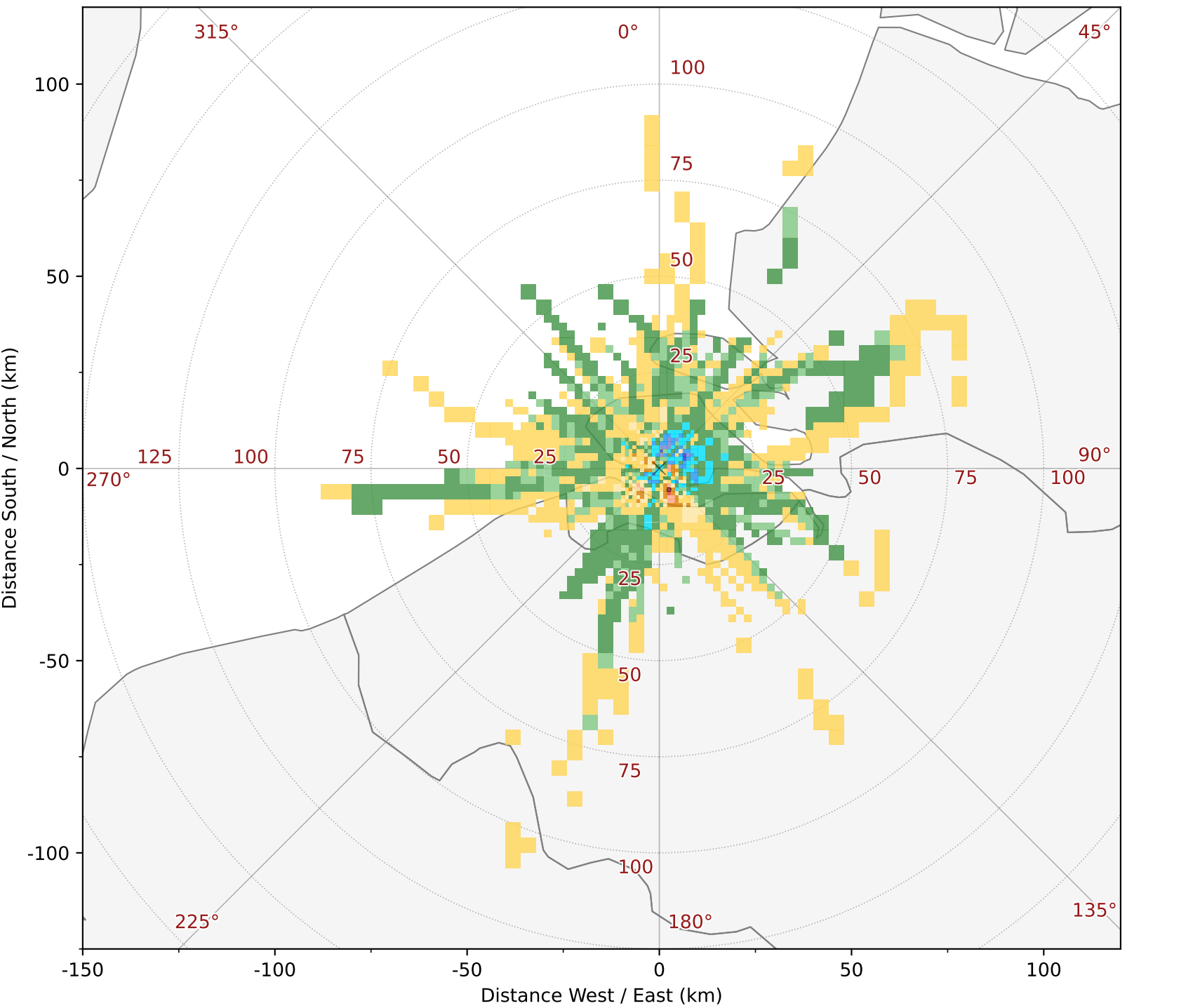
RIMPUFF-DIPCOT Difference Map - Evacuation. Min Cell Value: -0.0656, Max Cell Value: 0.0656
