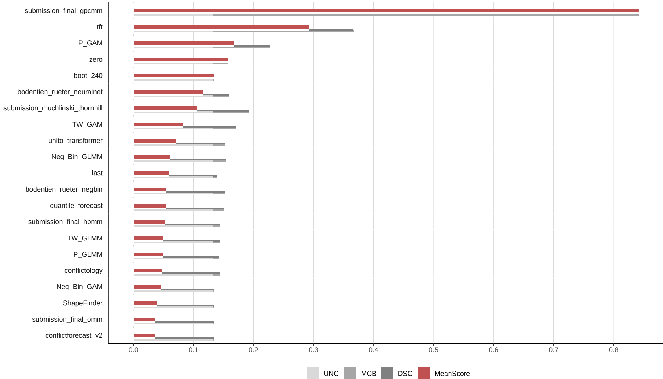
Mean Brier Score Decomposition for Onset Prediction (01–2018 to 12–2023, all countries)
