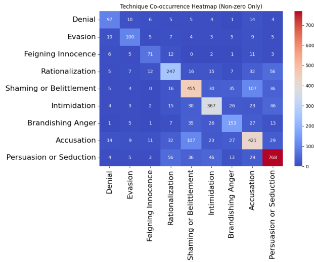
Figure A.4: Distribution and Co-occurrence of 'Manipulation Technique' labels
