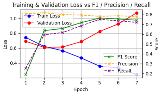
Figure 4: Losses and Results vs epochs (Note: the model is allowed to run beyond overfit at epoch 3 for illustration)
