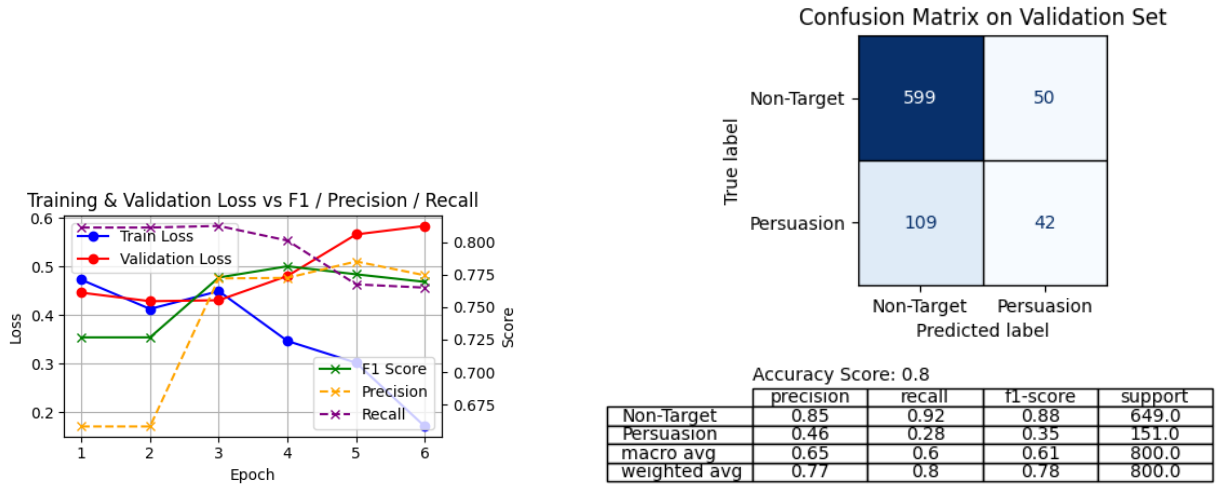
(a) Losses and Results vs epochs for the un-weighted model (b) Confusion matrix and classification report for the un weighted Persuasion label base case model
