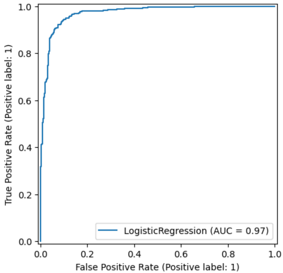
Figure 5: ROC curve
