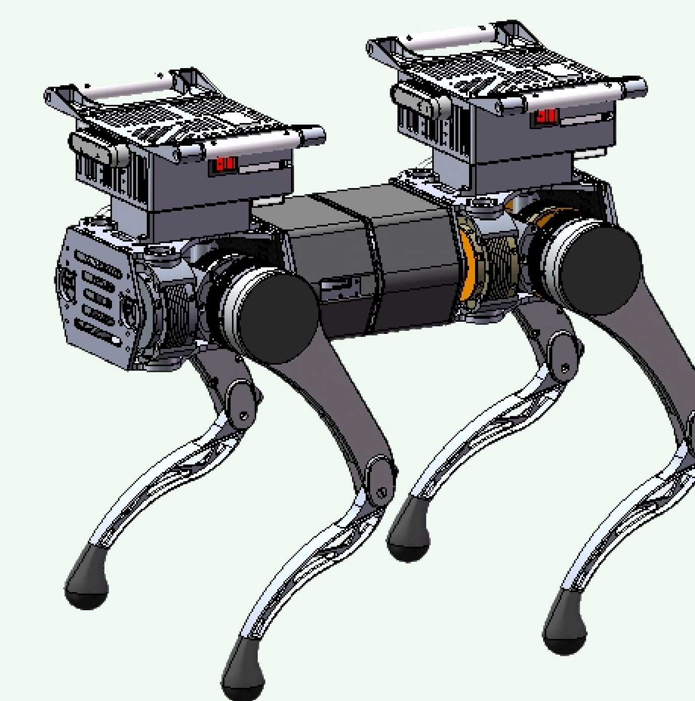
Quadruped
