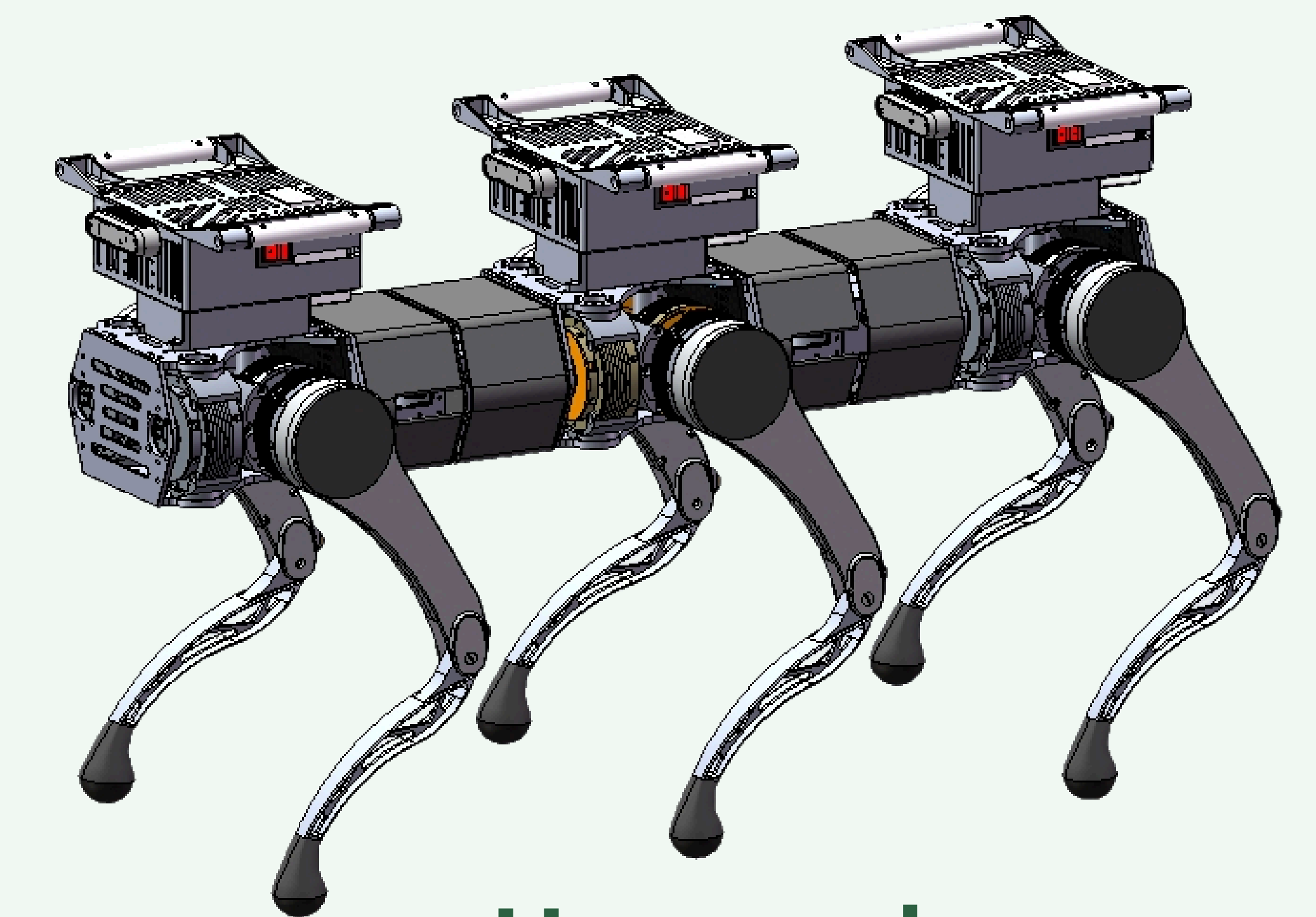
Hexapod
